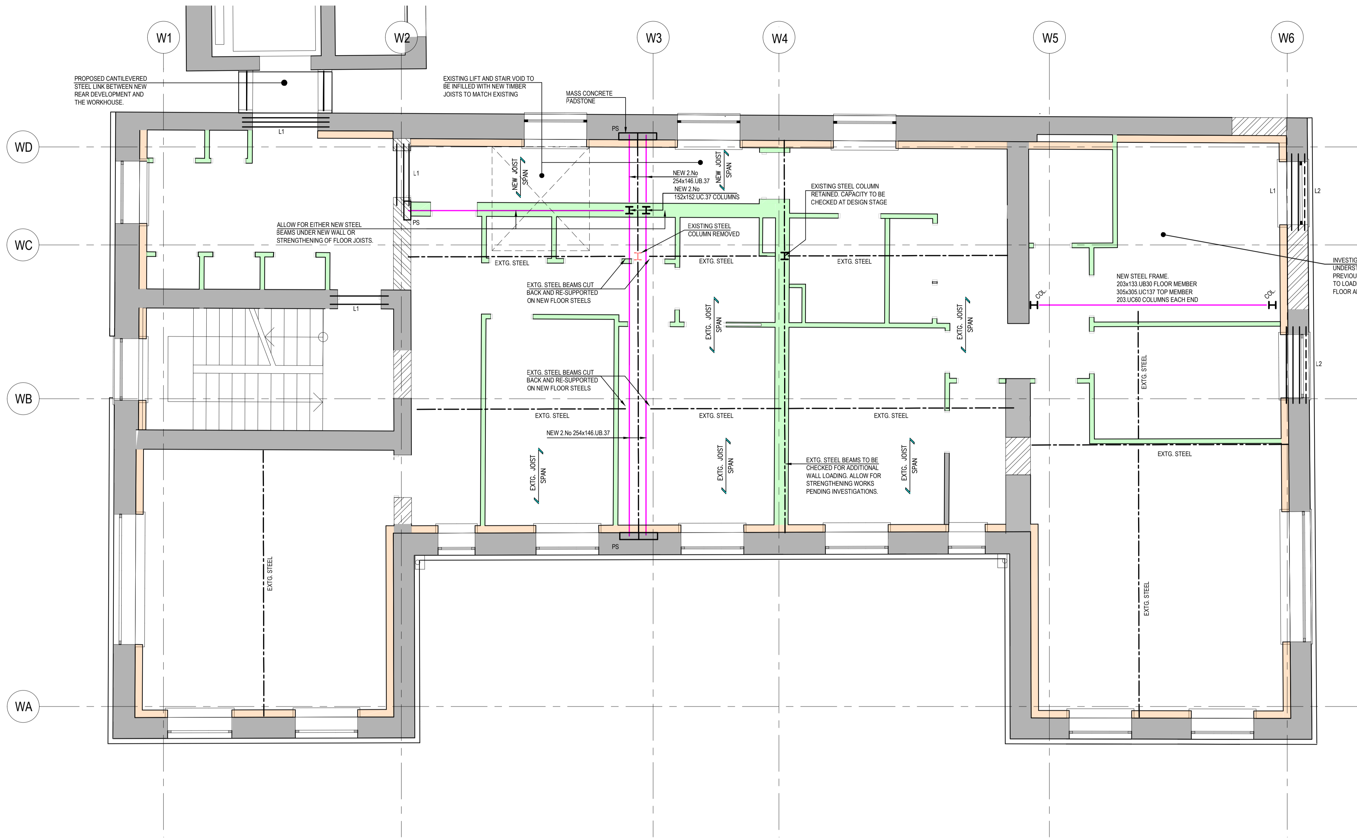
PROPOSED FIRST FLOOR PLAN [ LEVEL 01 ]
