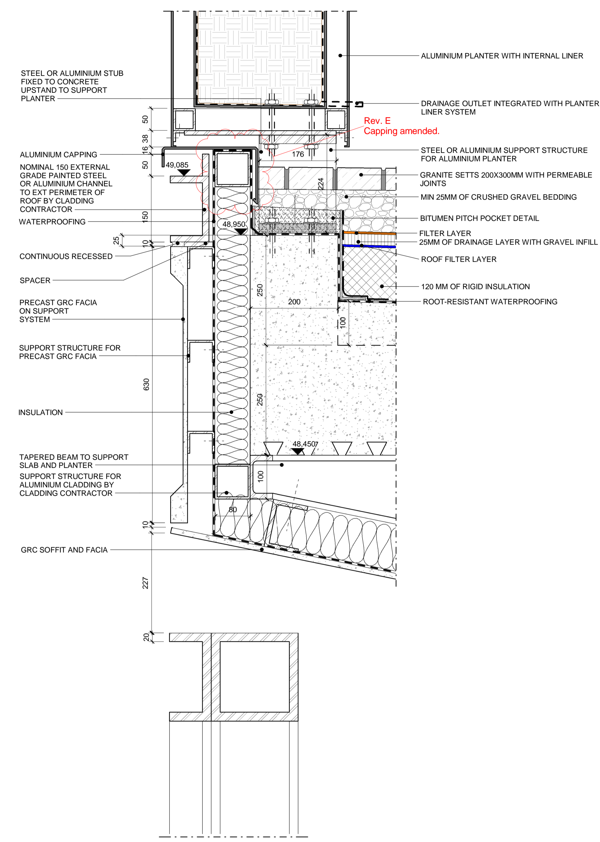
DET-C Roof Perimeter Detail-5th Floor 143218 1:5
