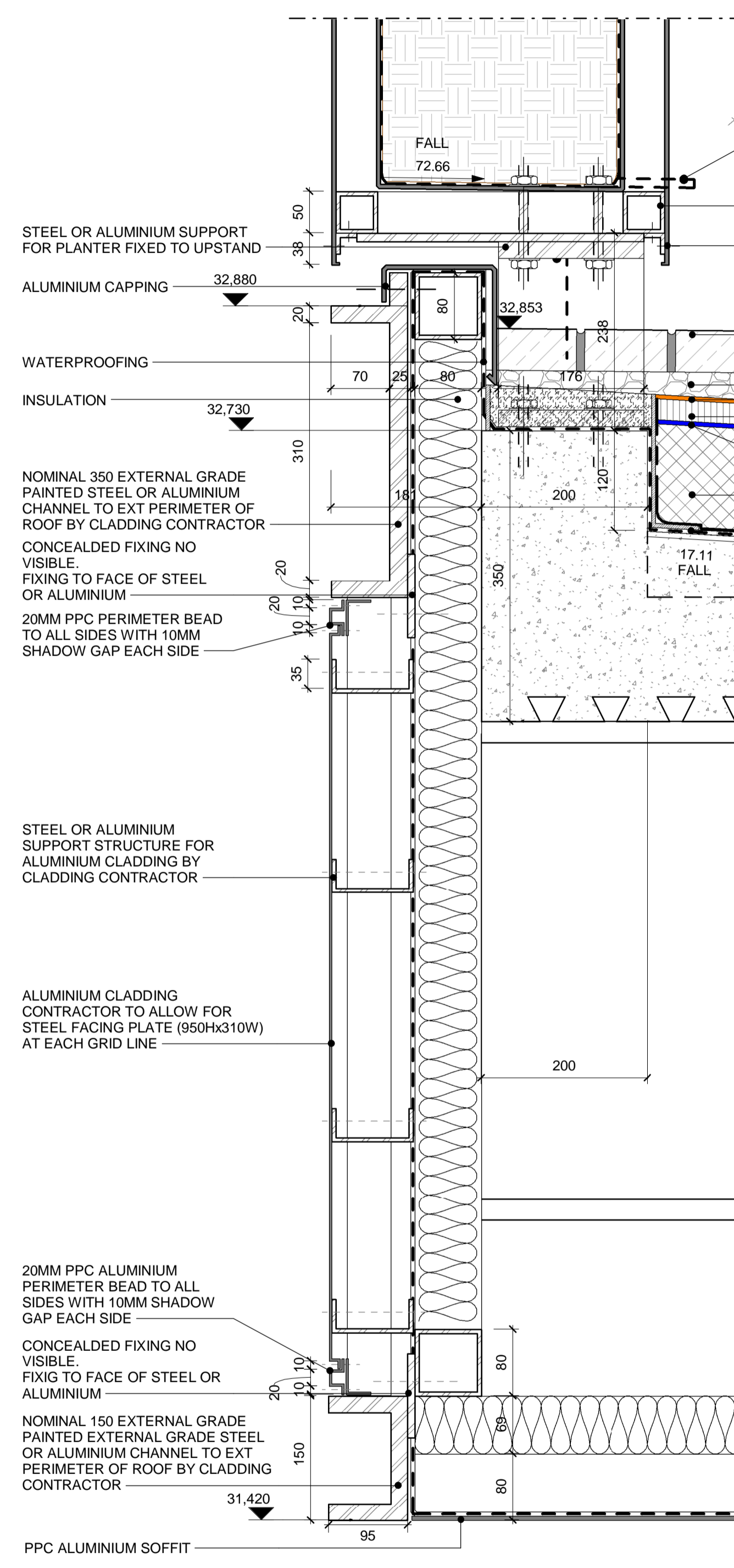
DET-A Roof Perimeter Detail-1st Floor 143218 1:5
