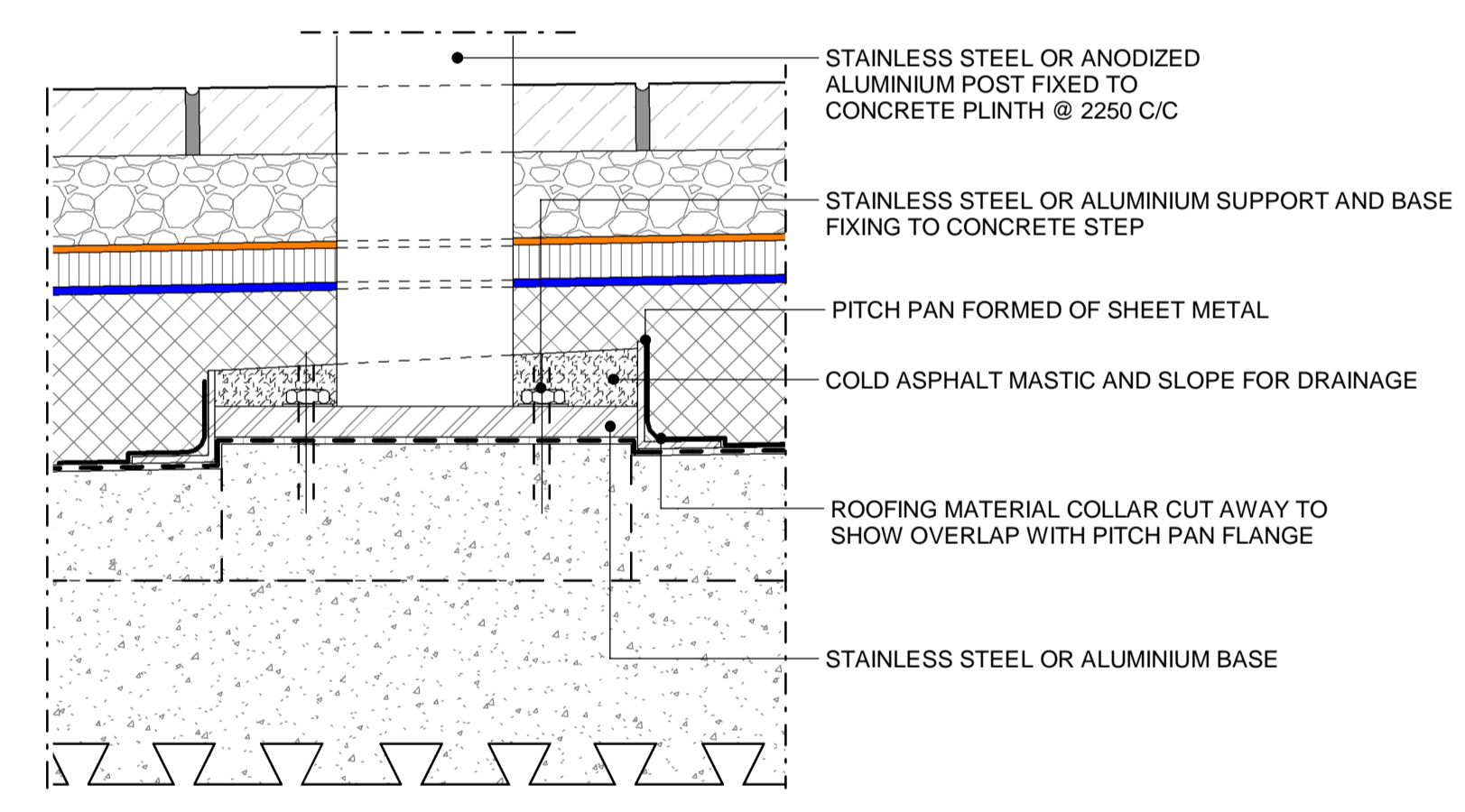
DET-F Pitch Pocket Detail 143219 1:5
