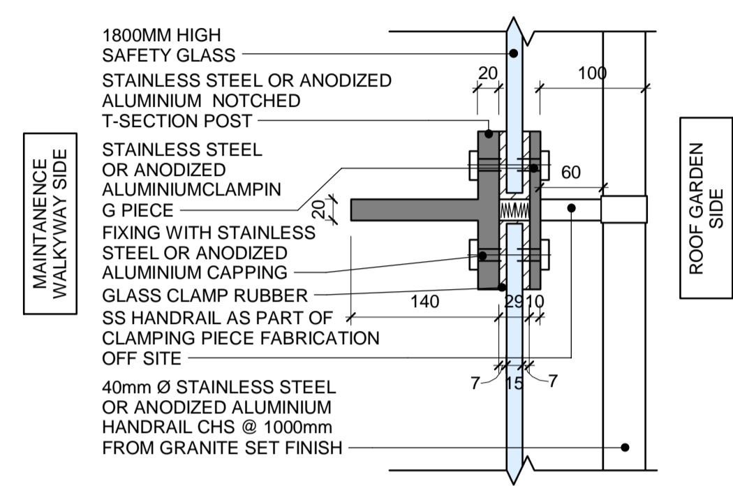
DET-E External Balustrade Post Plan Detail 143219 1:5
