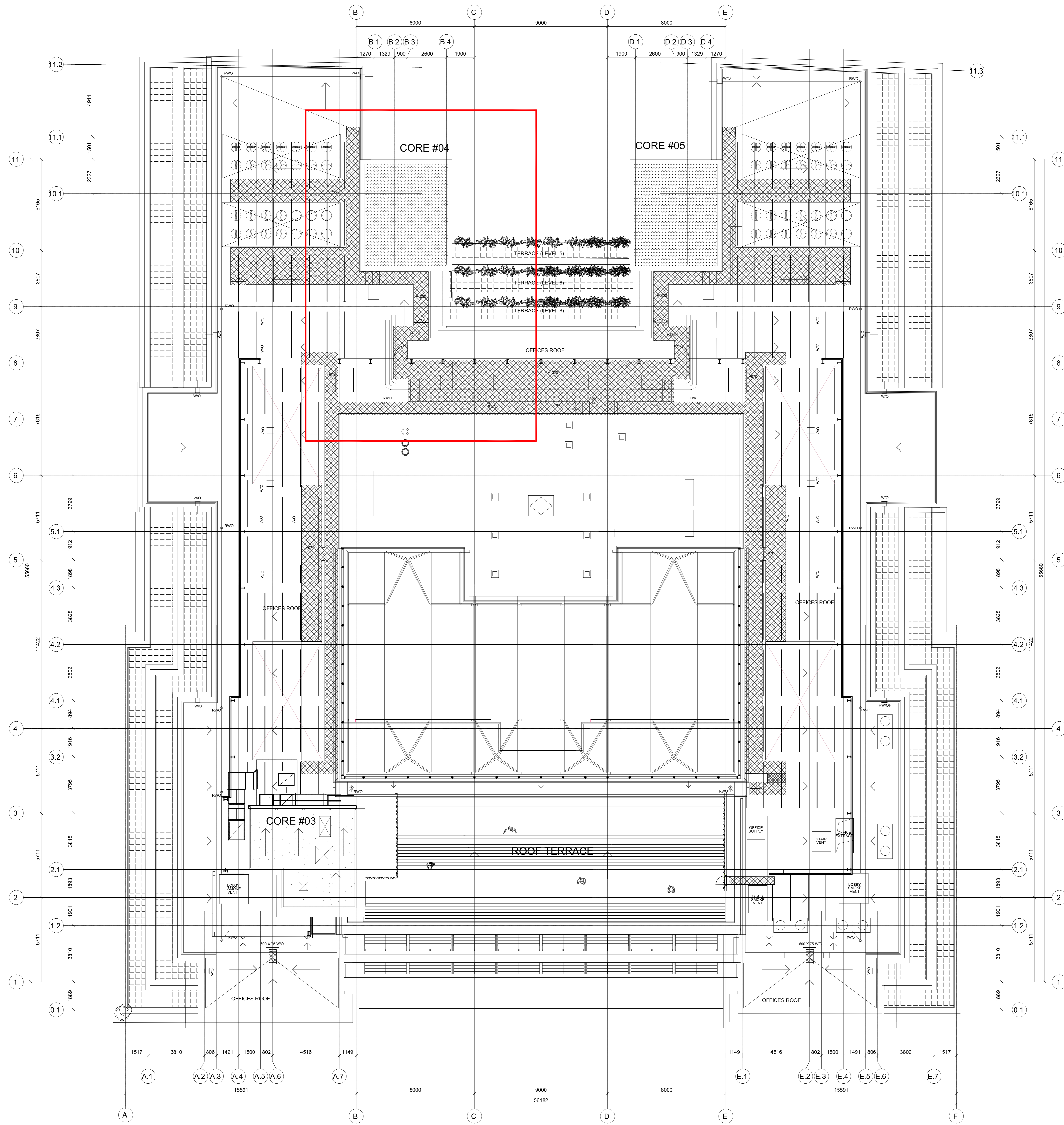
1 ROOF LEVEL PLANT LOCATION Scale: 1:100
