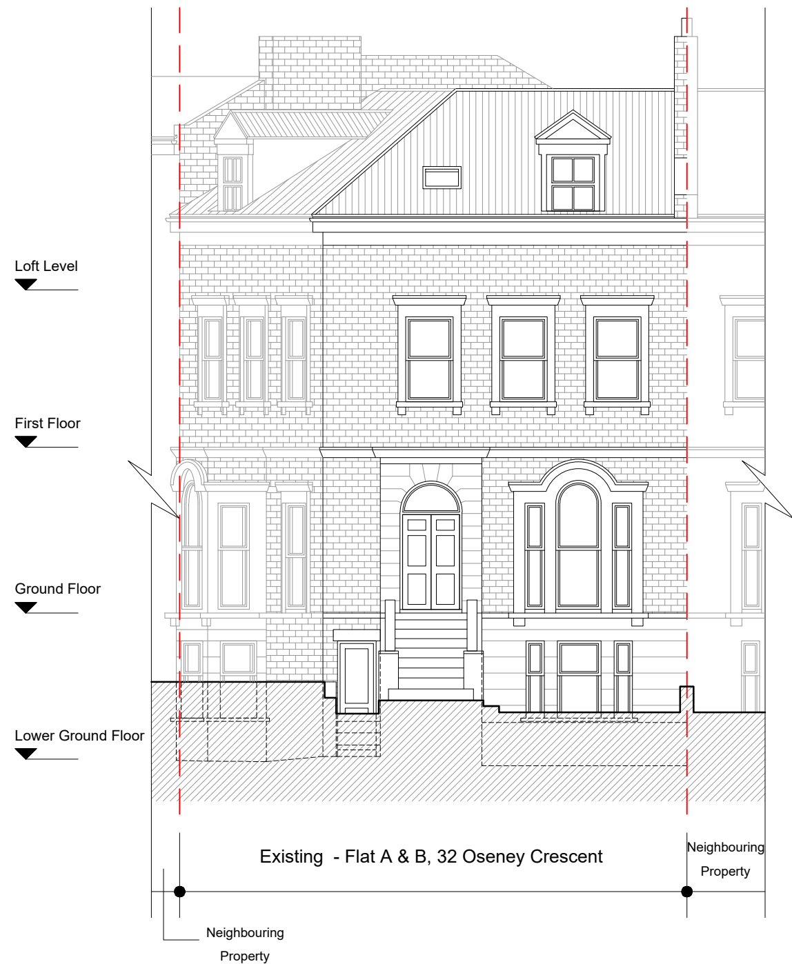
Front Elevation
