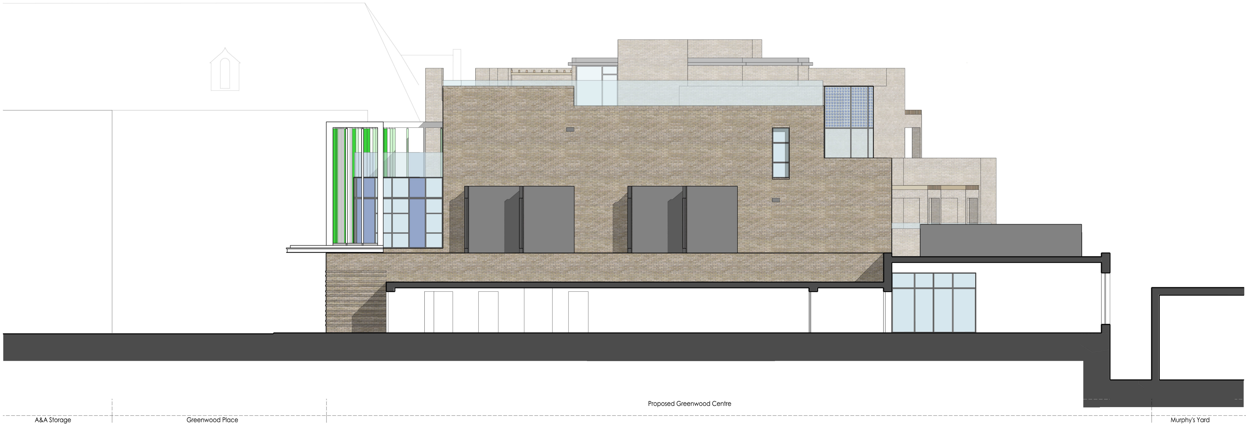
WEST ELEVATION 4-4
