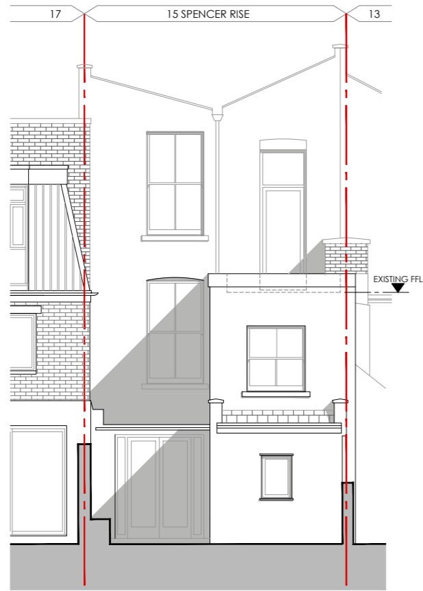
1 ELEVATION - REAR EXISTING 1:100
