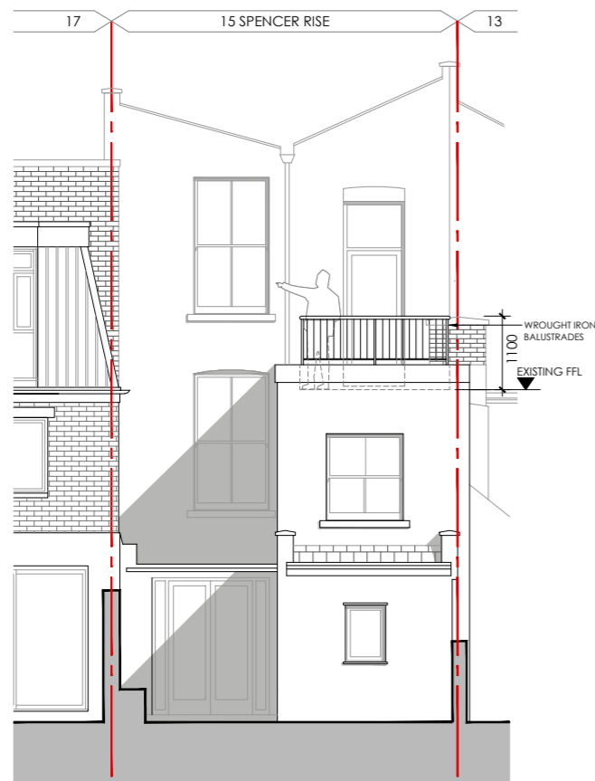
3 ELEVATION - REAR PROPOSED 1:100
