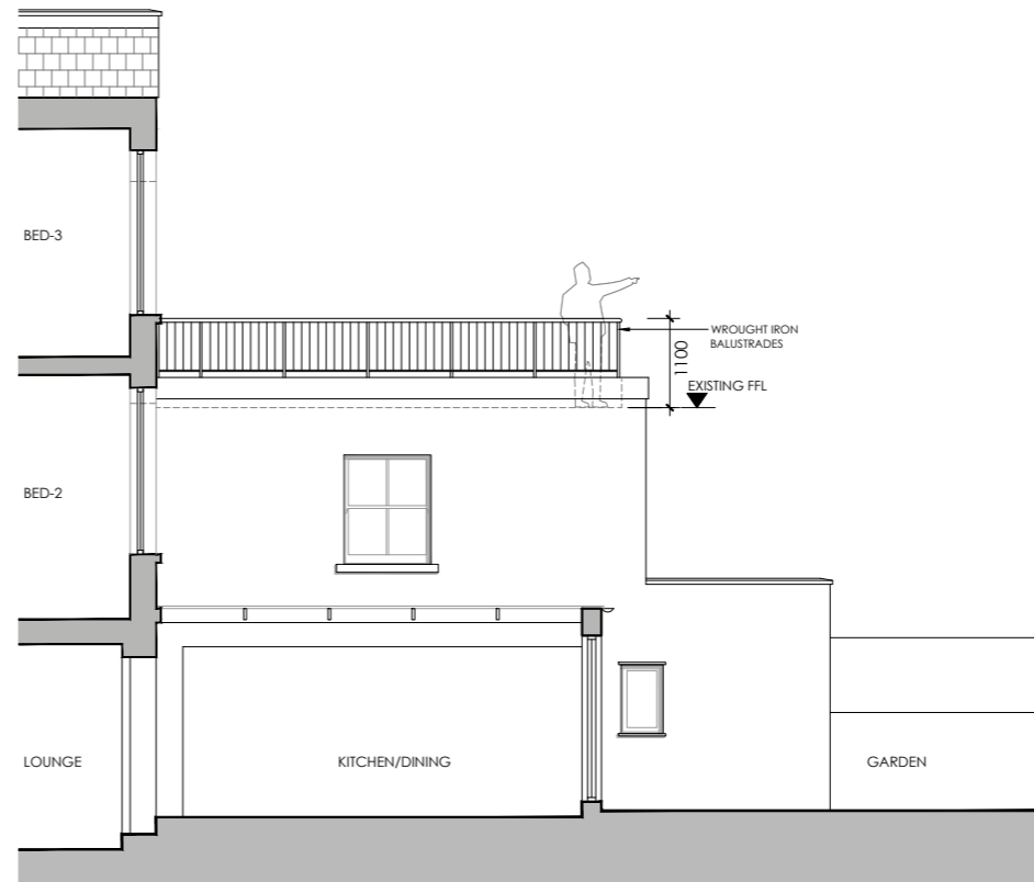
4 ELEVATION - SIDE PROPOSED 1:100
