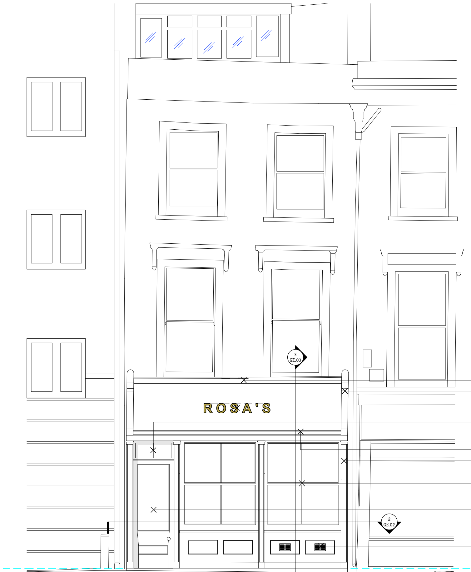
1 Proposed Shop Front Elevation 1:50@A3
