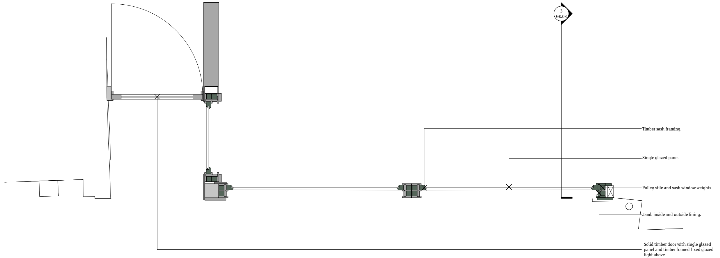
2 Proposed Shop Front Detailed Plan 1:20@A3
