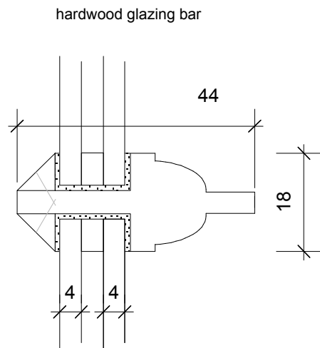
A GLAZING BAR DETAIL 1:1
