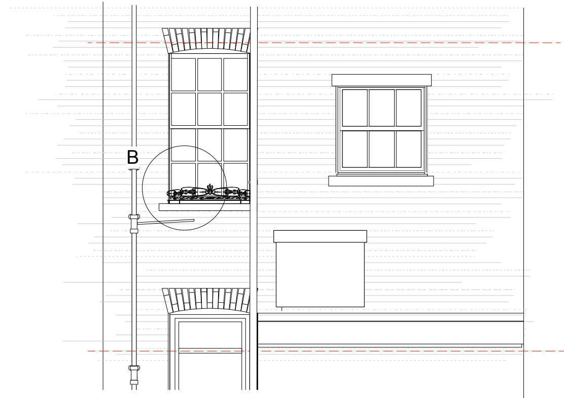
SIX OVER SIX SASH WINDOW
