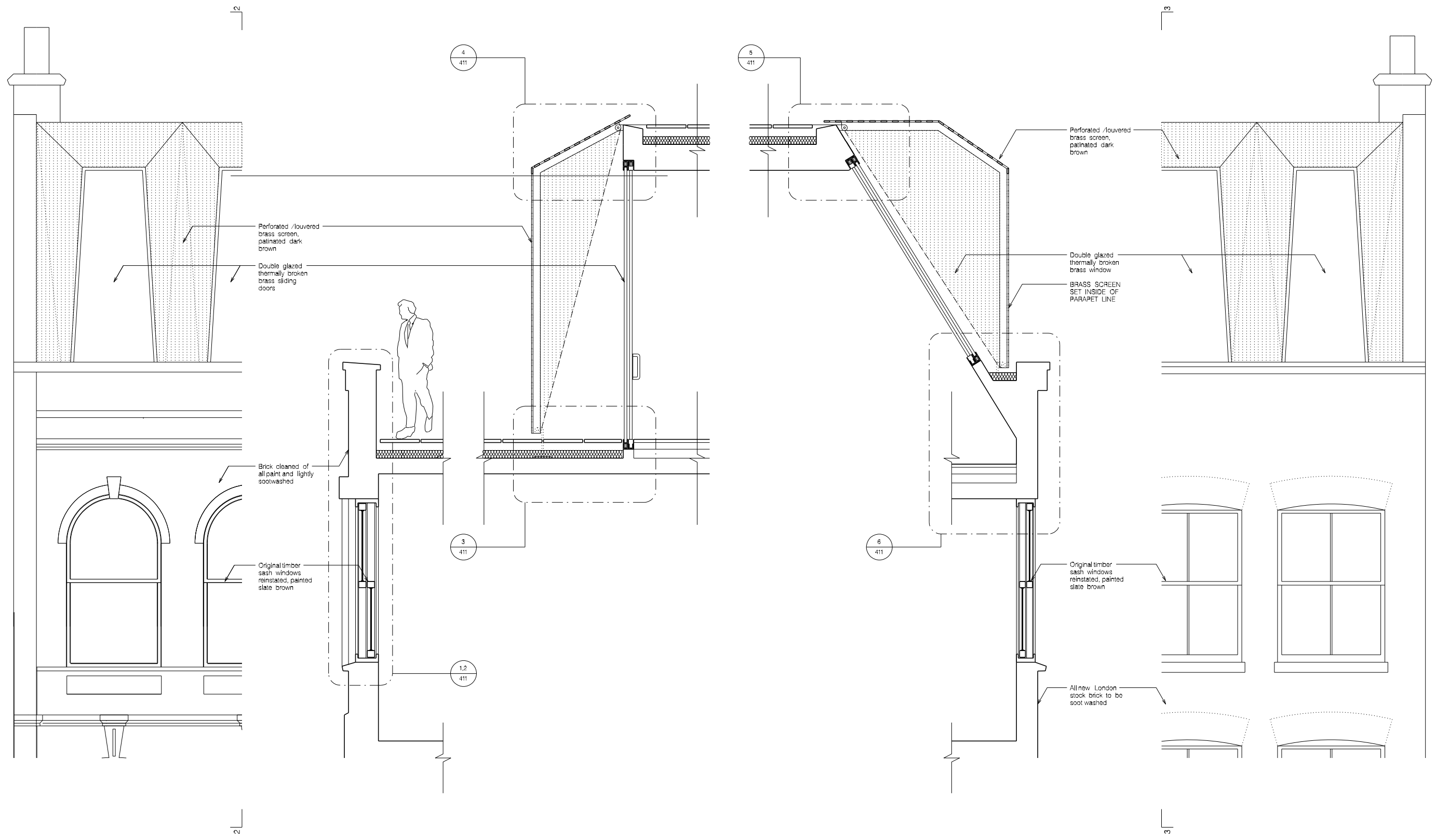
① PROPOSED ROOF DETAIL FRONT ELEVATION
