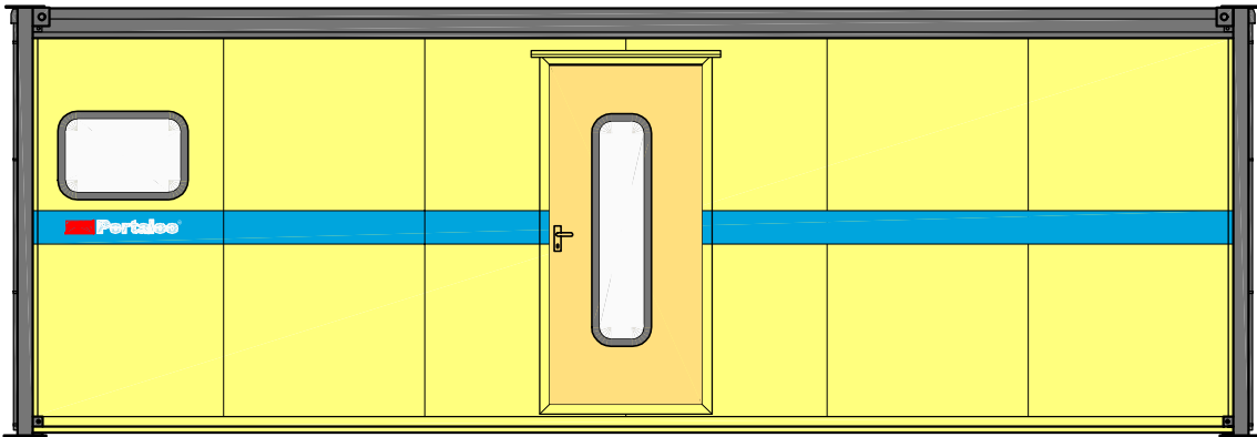
SIDE ELEVATION
