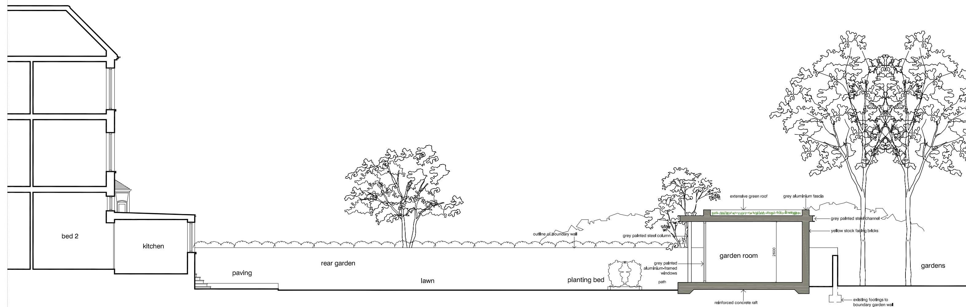
section AA as proposed
