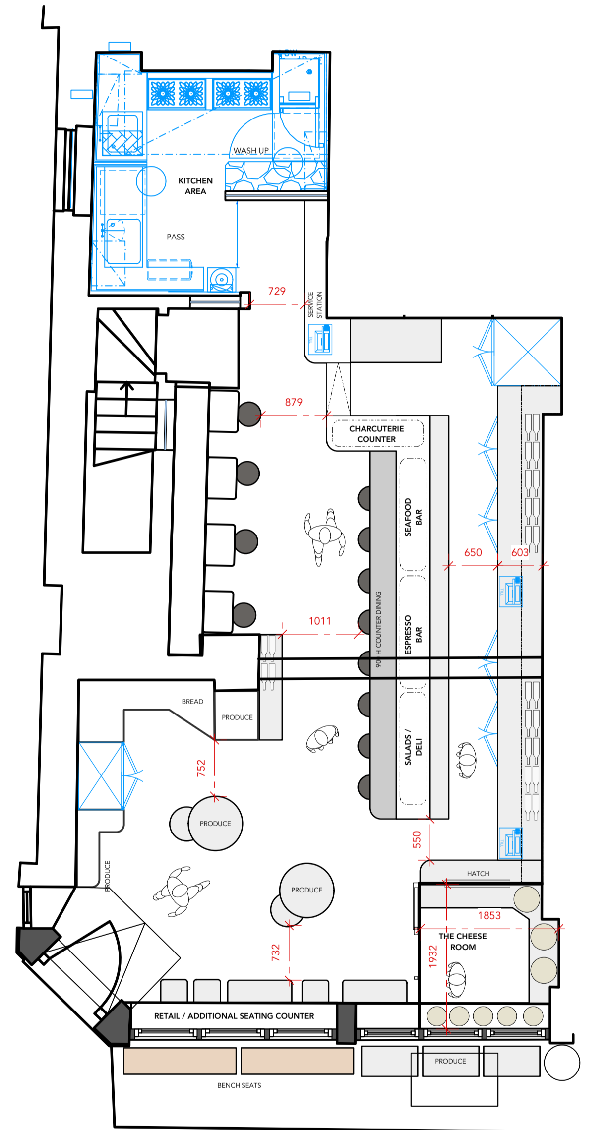
1 GROUND FLOOR SCALE 1:50 @ A1, 1:100 @ A3
