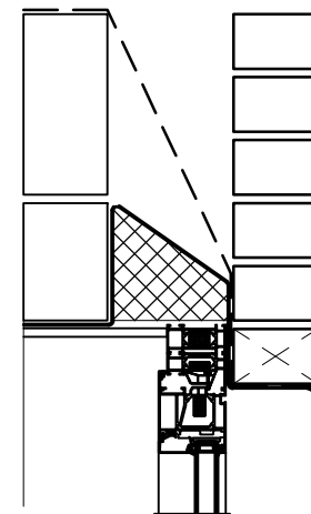
Head Detail Scale 1:10
