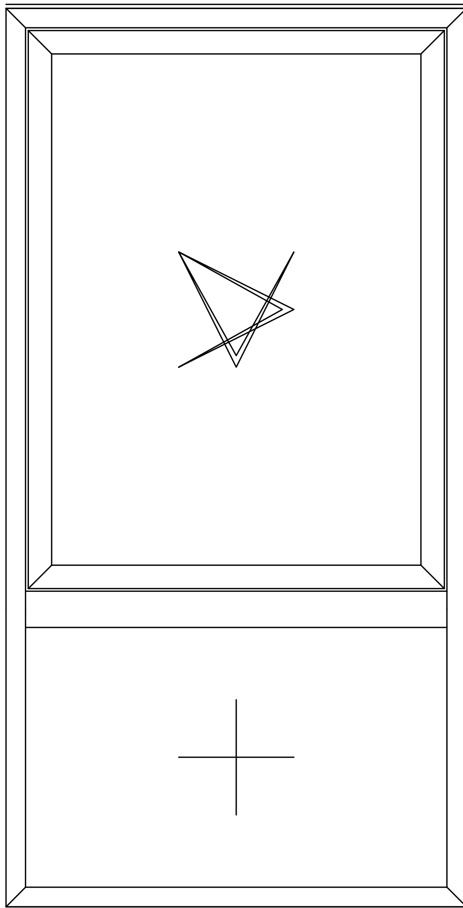
Elevation Scale 1:10
