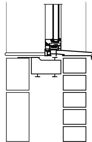
Cill Detail Scale 1:10
