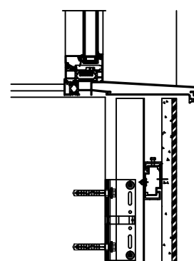
Cill Detail Scale 1:10
