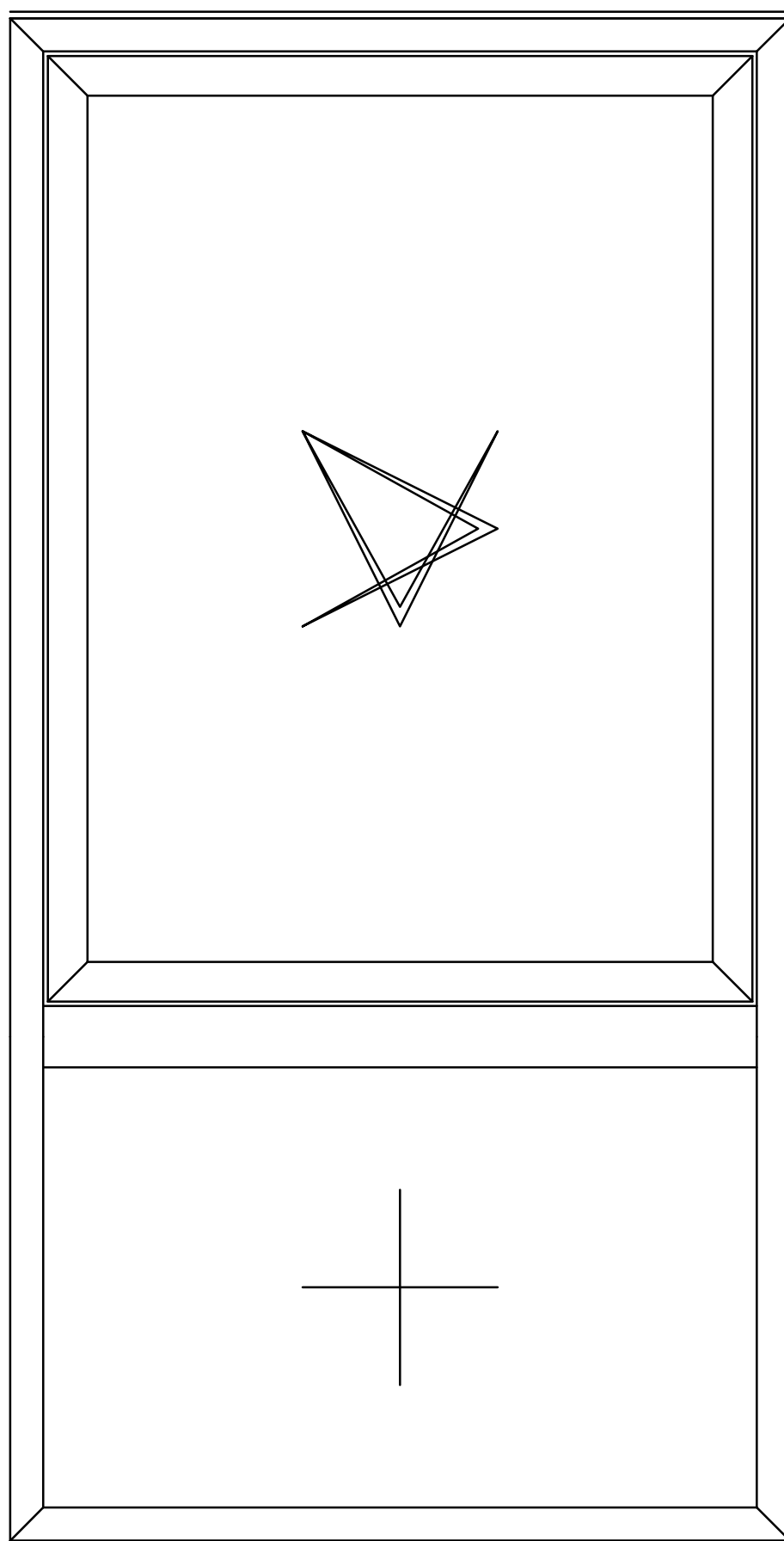
Elevation Scale 1:10
