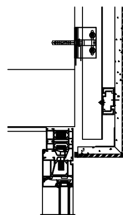
Head Detail Scale 1:10
