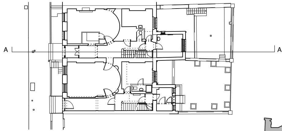
KEY PLAN
