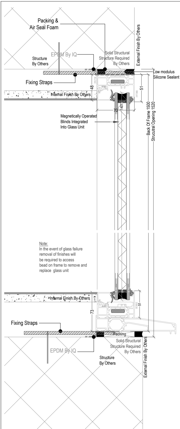
5.00 B1-B1 Section Detail - Summer Room Scale 1:2
