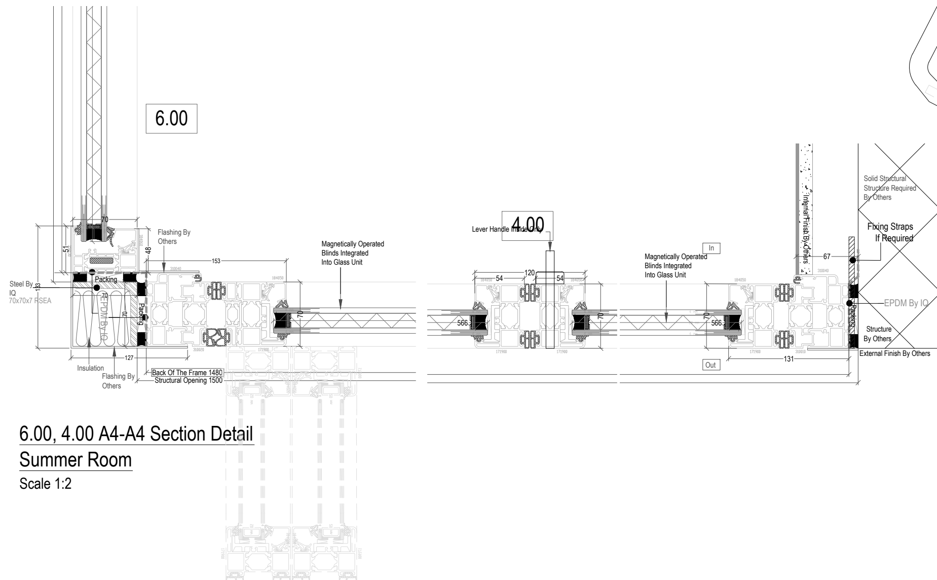
5.00, 3.00, 6.00 A4-A4 Section Detail - Summer Room Scale 1:2
