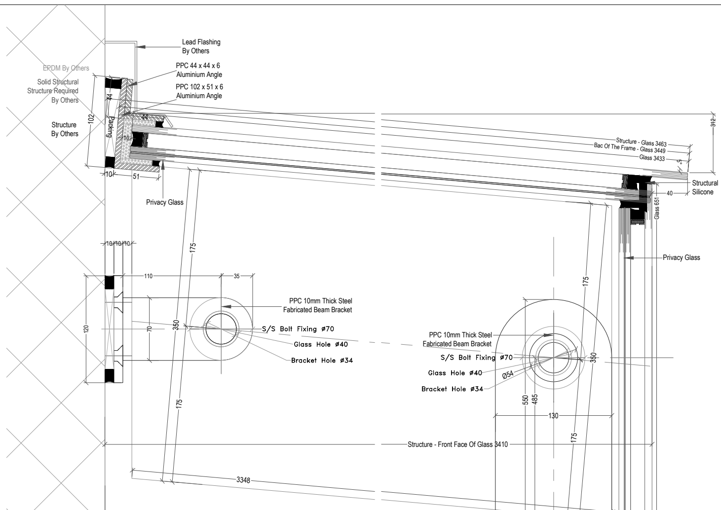
1.00, 2.00, 7.00 B-B Section Detail Scale 1:2
