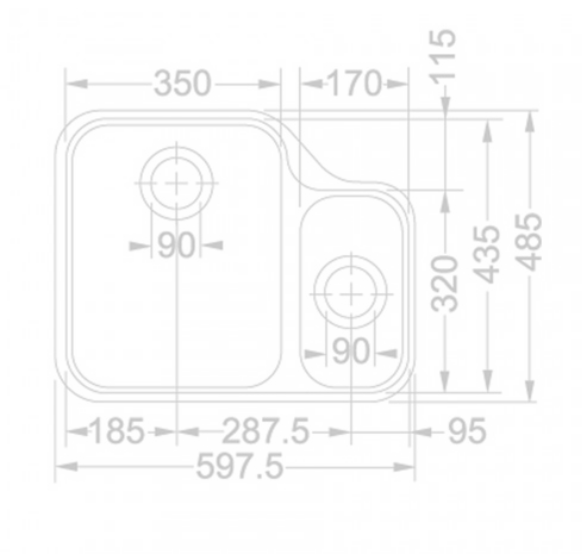
Stainless Steel 1.5 bowl Sink Duo Undermount e.g. Franke Ariane ARX 160
