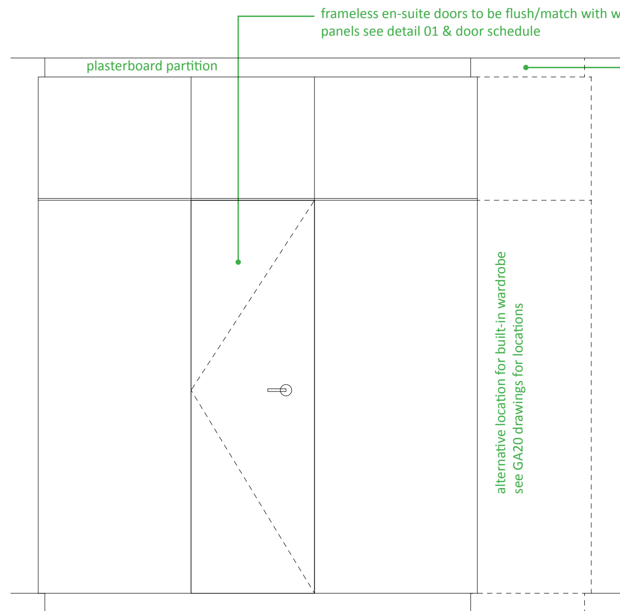
Elevation A (1:20)
