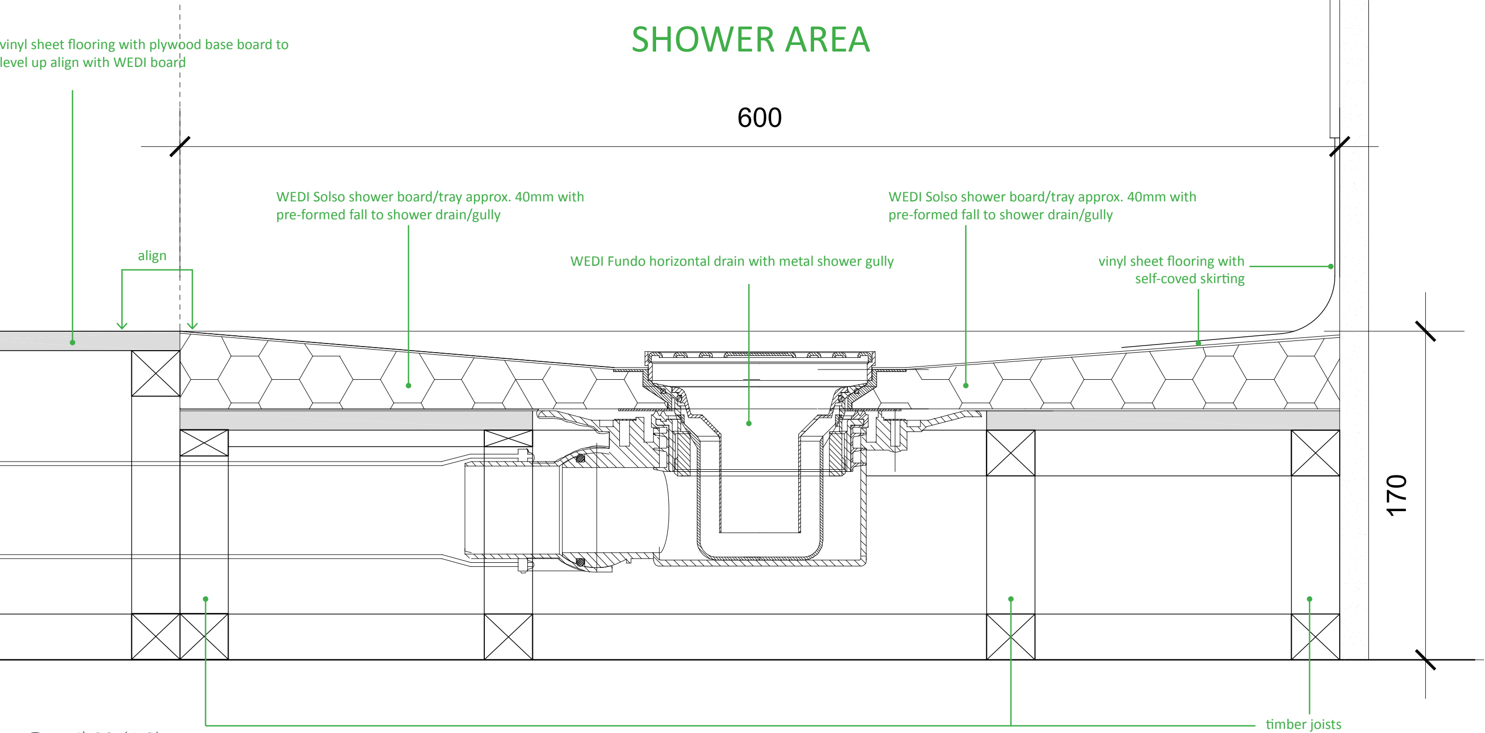
Detail 03 (1:2)
