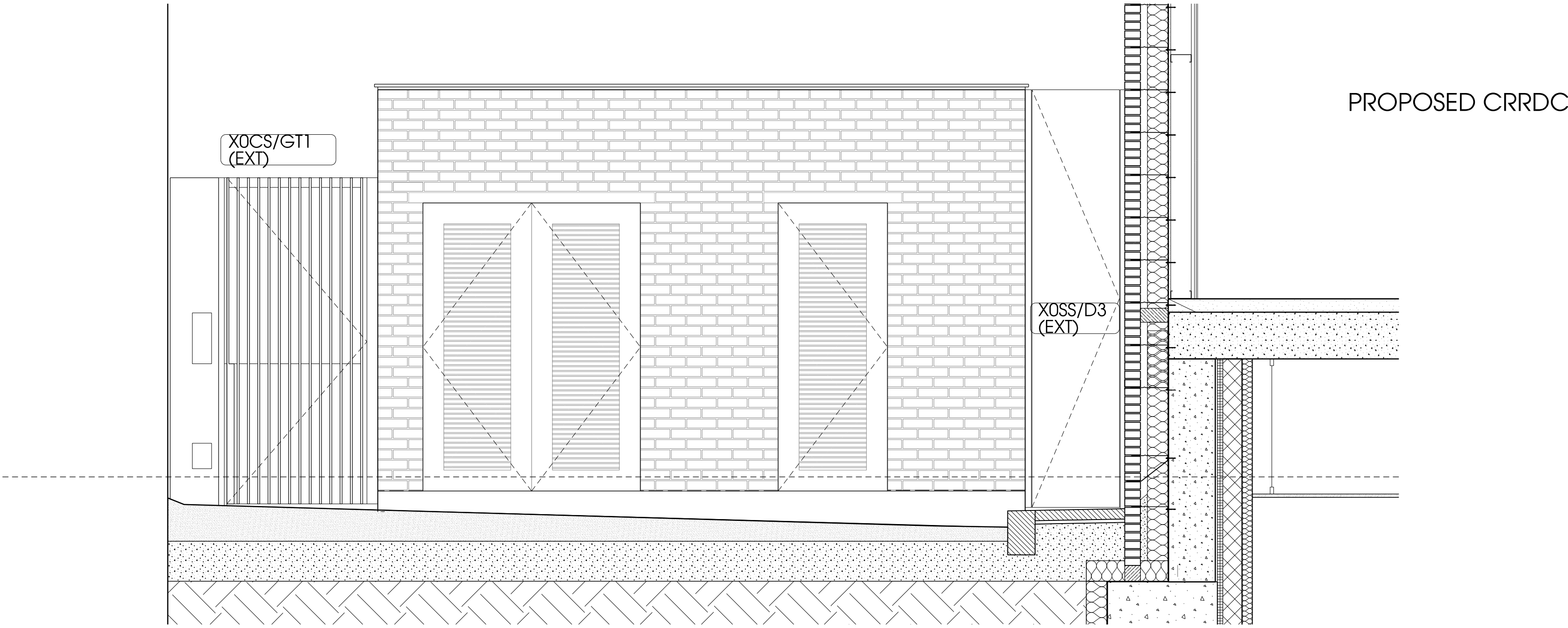
01 Substation East Elevation SK_1932 Refer to Drawing 90_300
