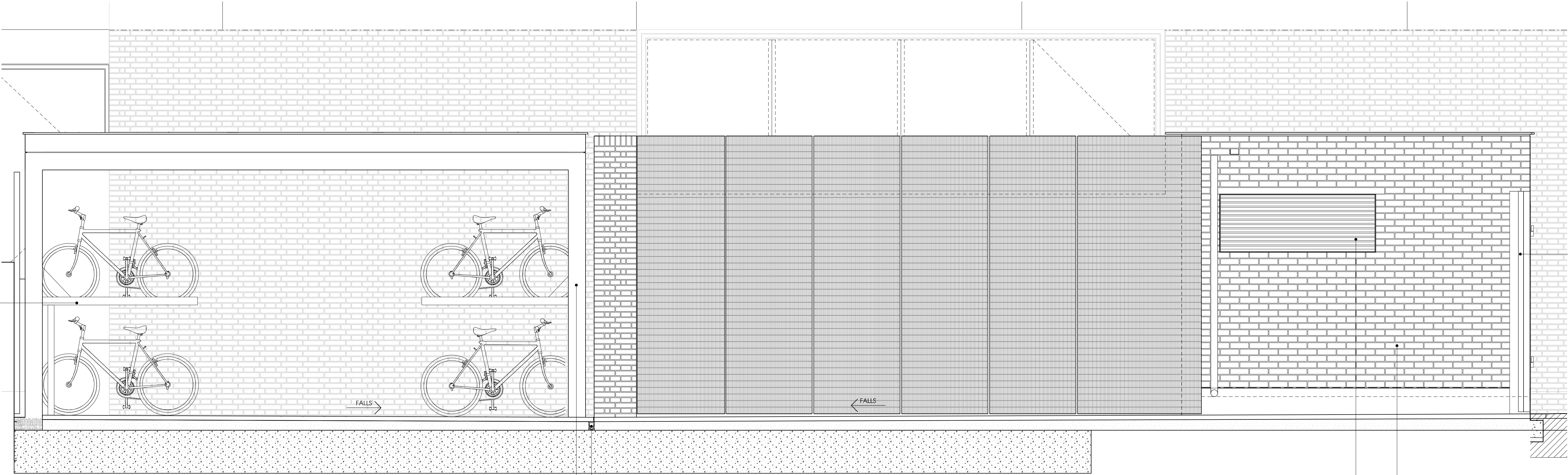
01 Substation East Elevation SK_1932 Refer to Drawing 90_300
