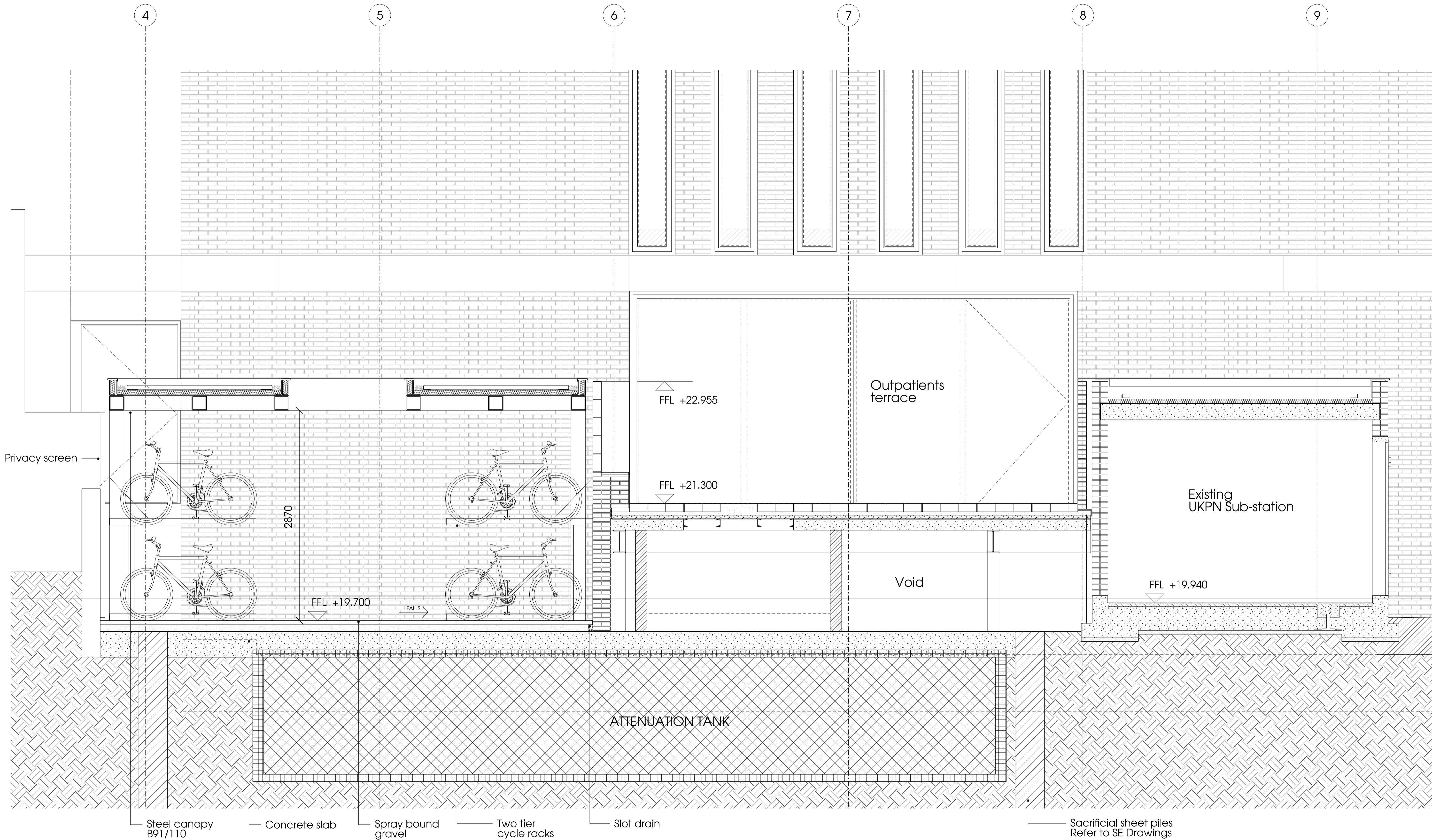
01 Cycle store / Substation Proposed Long section SK_1931 Refer to Drawing SK_1930
