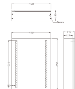
Lower Profile Shower Tray
