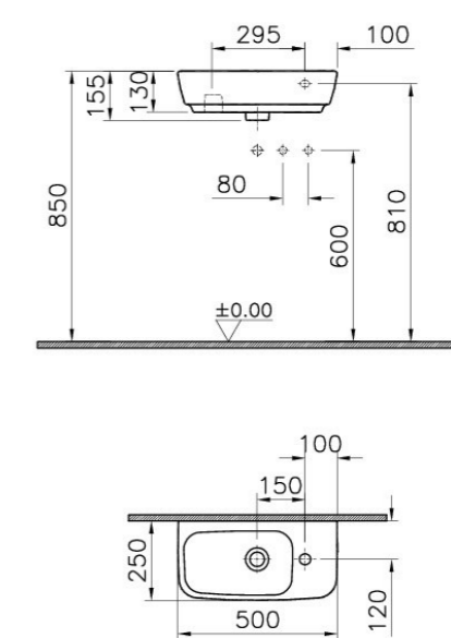
Compact Wall hung Washbasin (Chrome pop up waste) e.g. Vitra Shift 4387B003-0921
