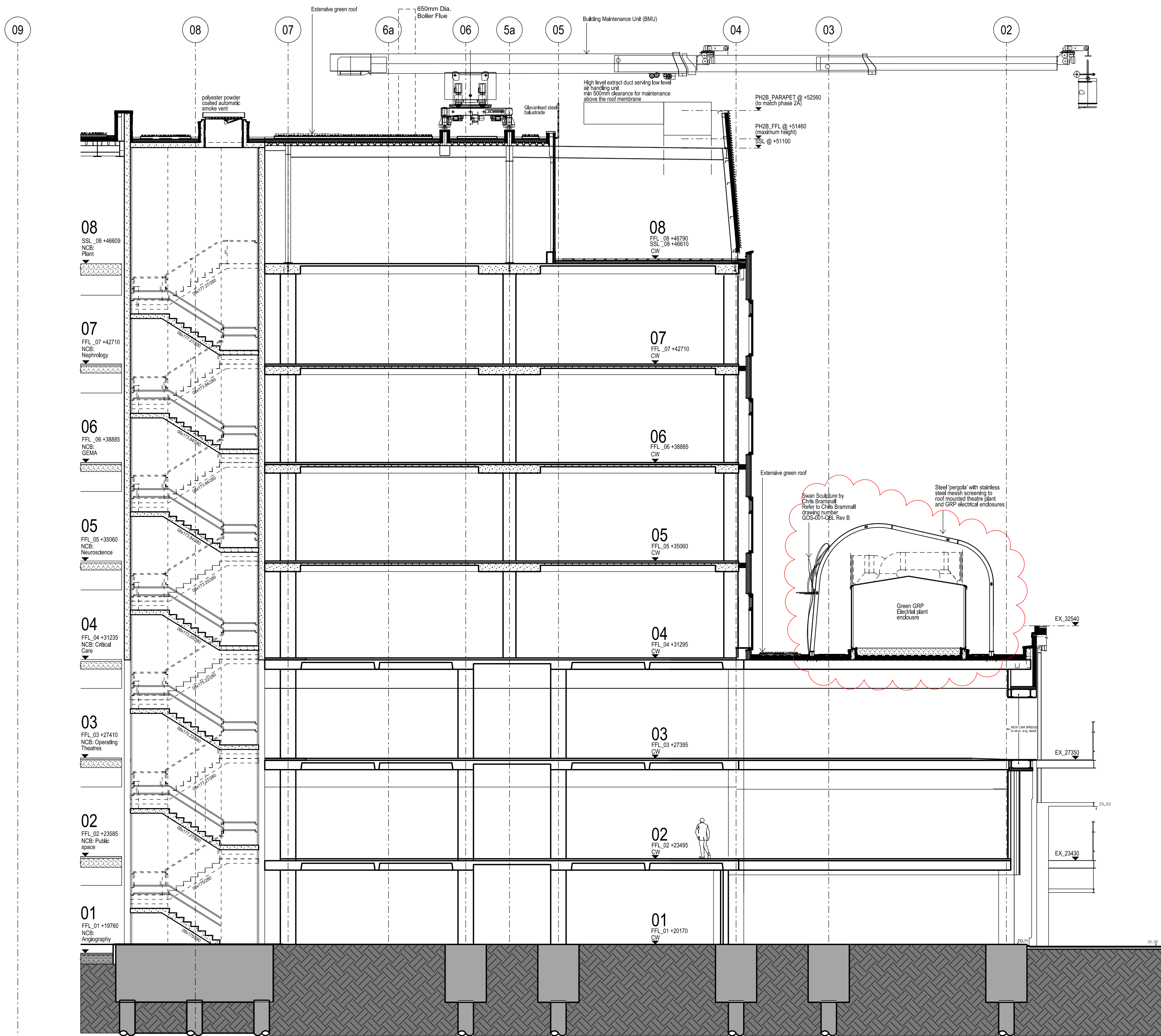
SECTION E-E
