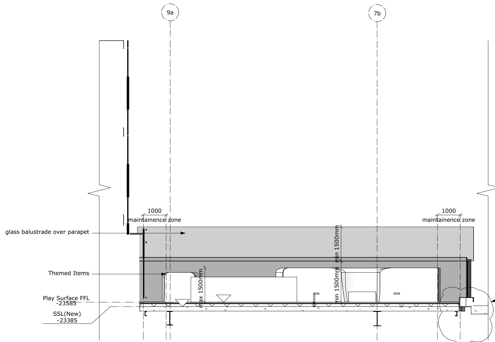
01 Elevation - North (Facing Balustrade)
