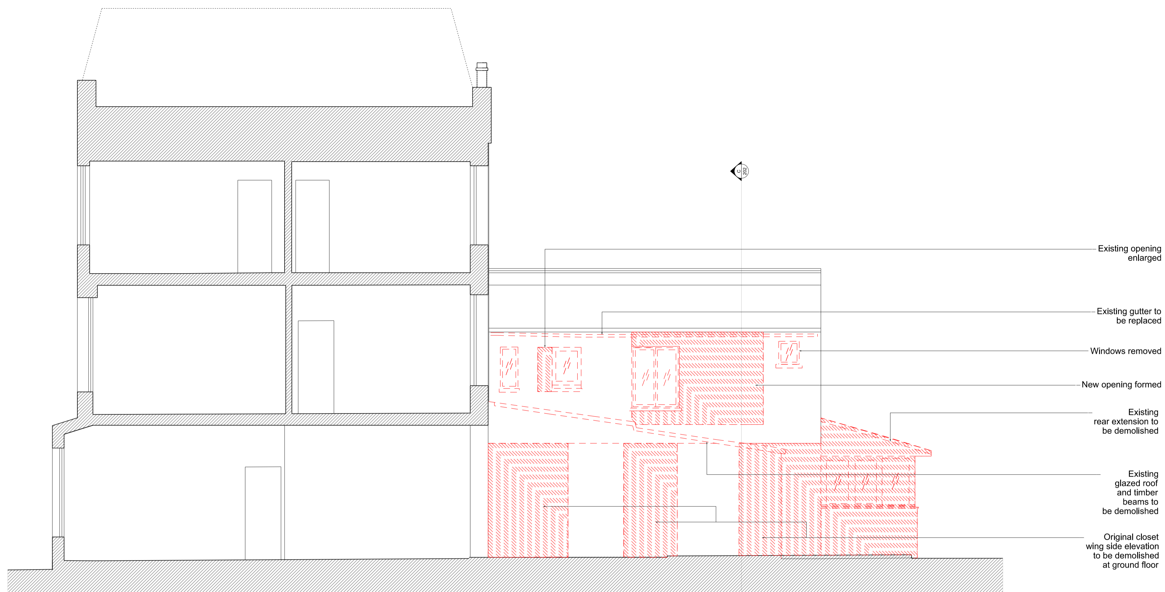
EXISTING & DEMOLITION SECTION B-B
