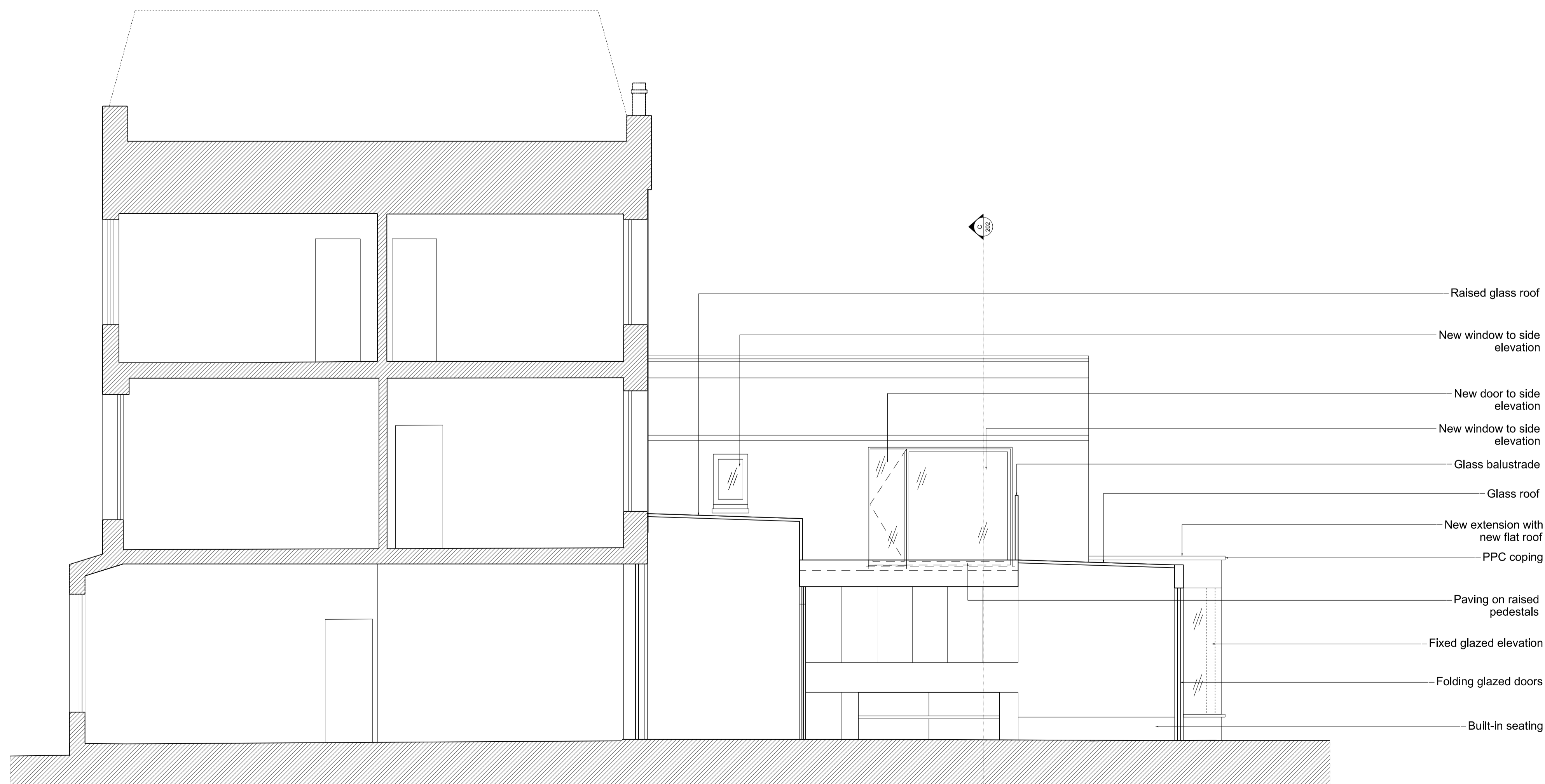
PROPOSED SECTION B-B
