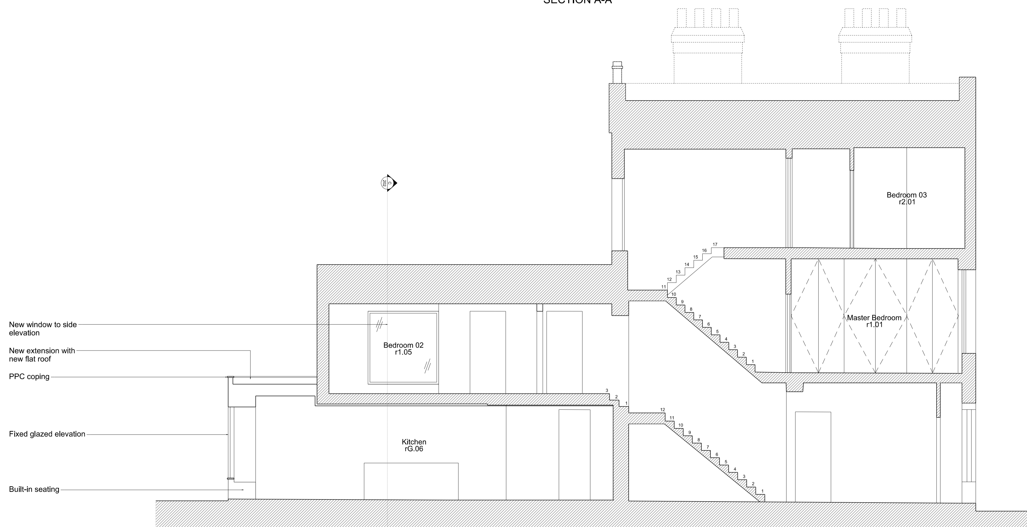
PROPOSED SECTION A-A
