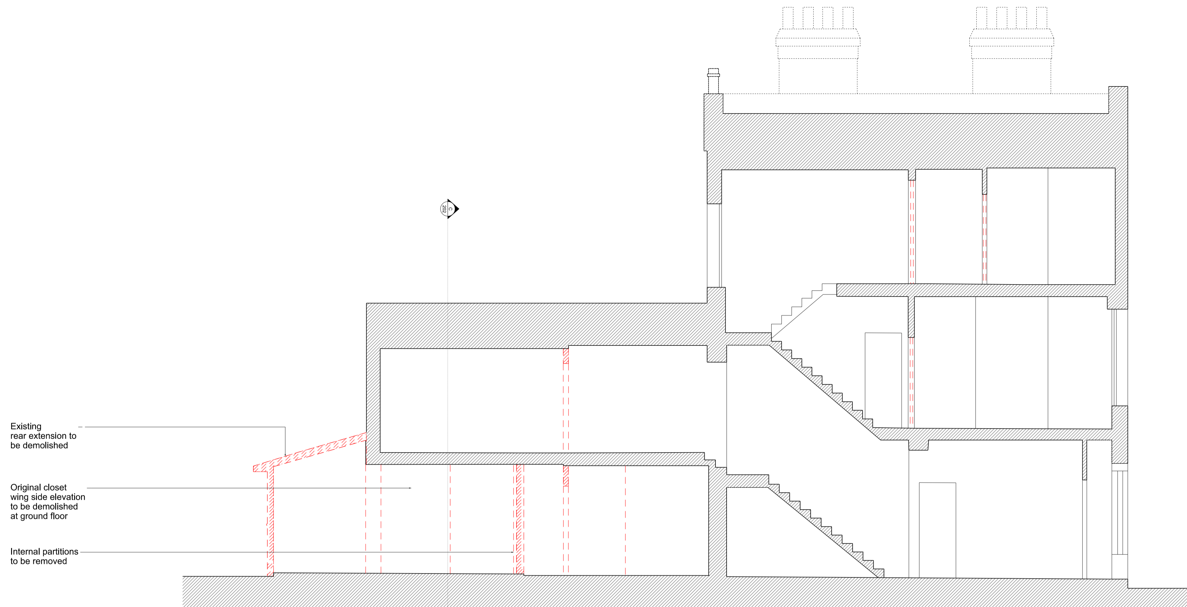
EXISTING & DEMOLITION SECTION A-A
