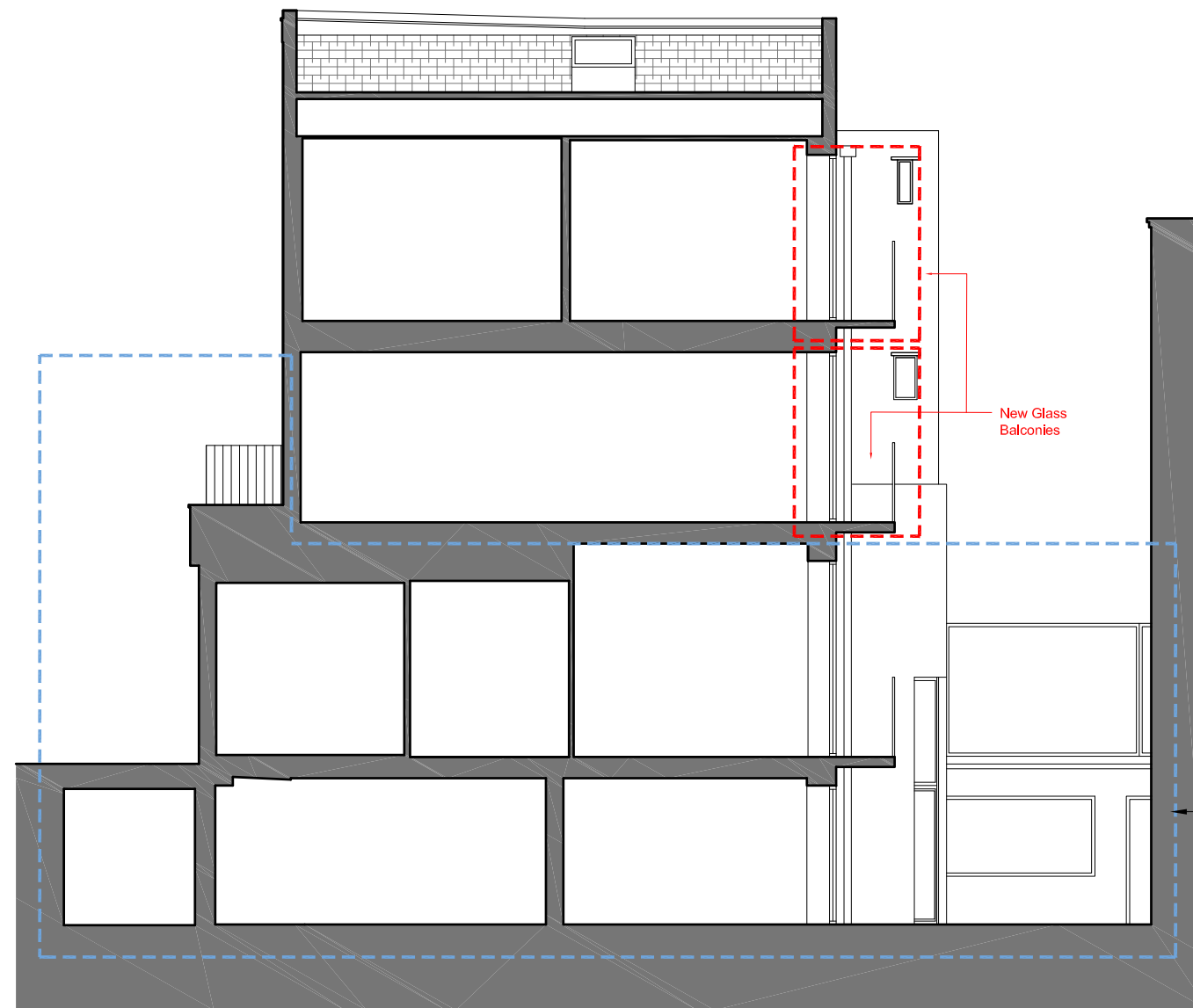
01 Section A
