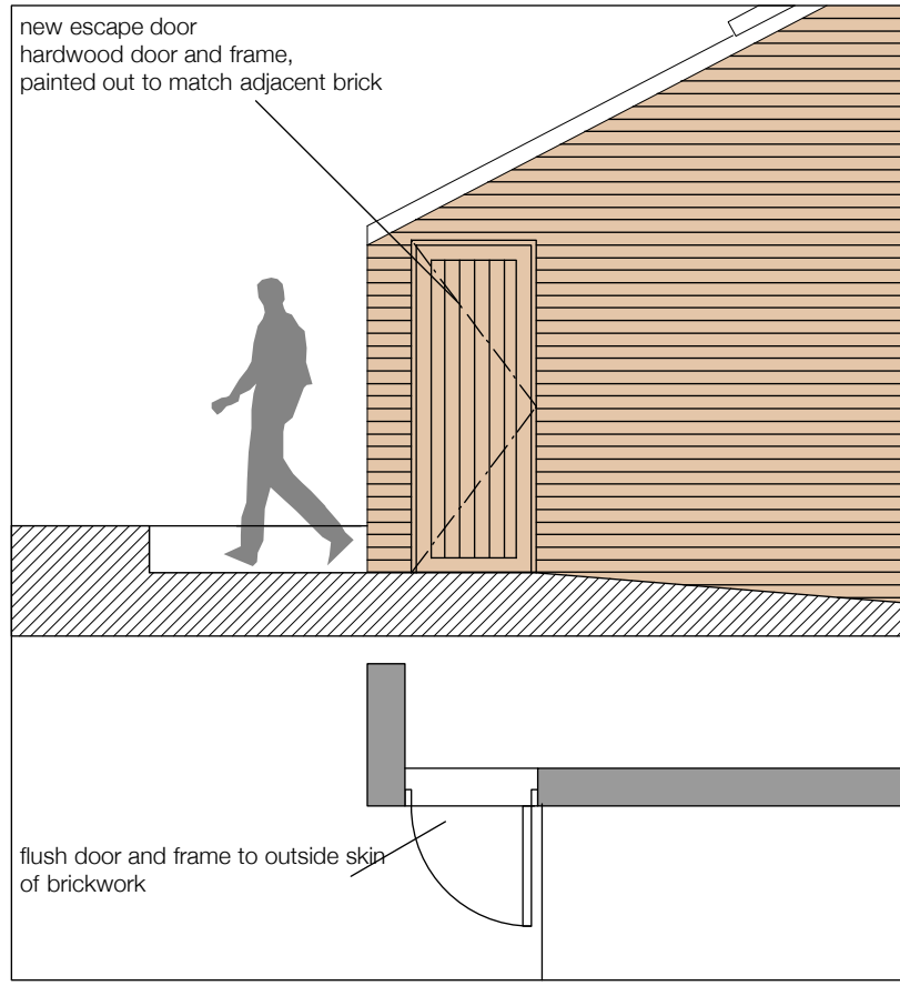
extract of elevation 1:50
