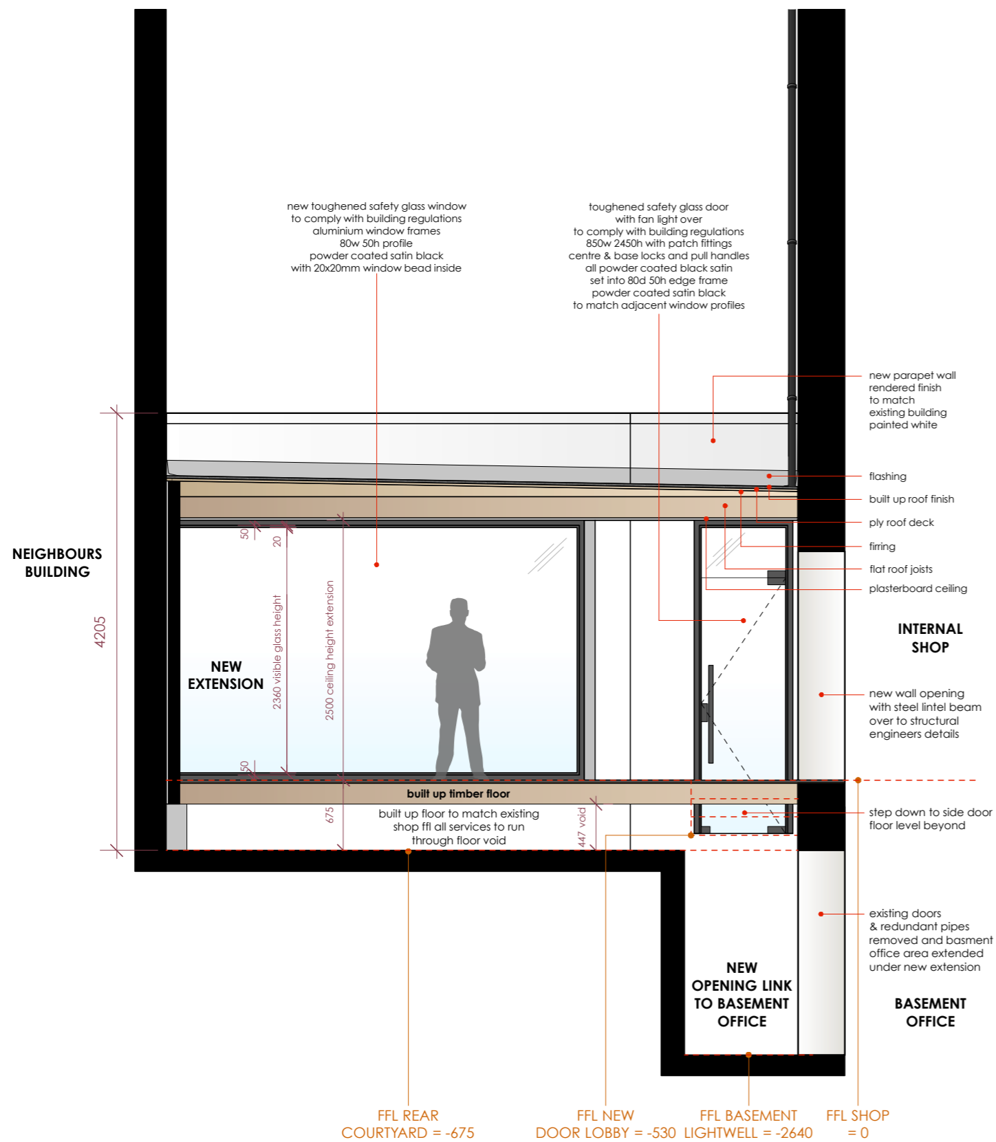
proposed SECTION EE
