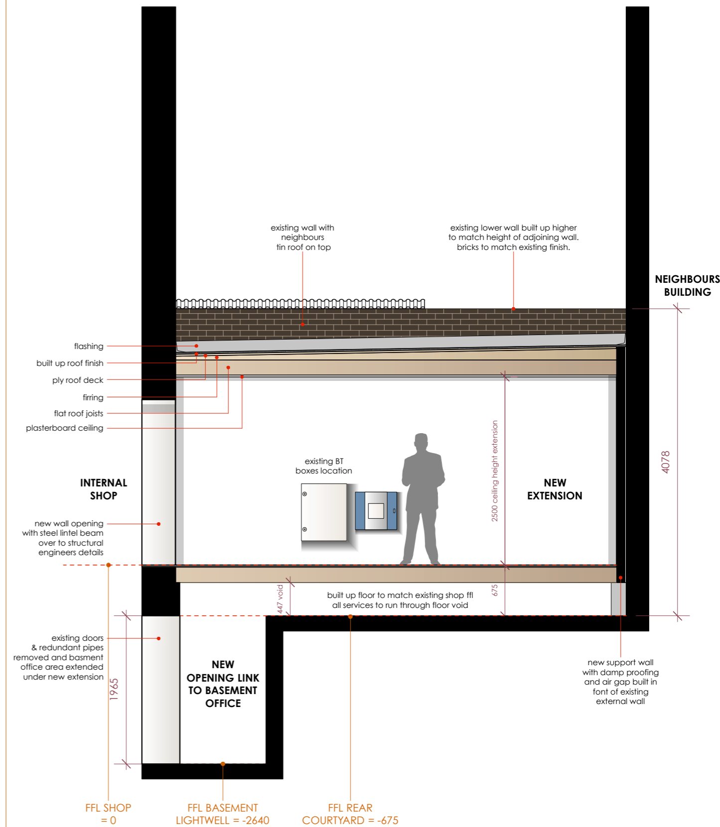
proposed SECTION DD
