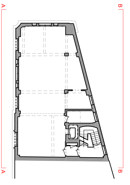
C Key Plan 1:250 @ A1 1:250 @ A1
