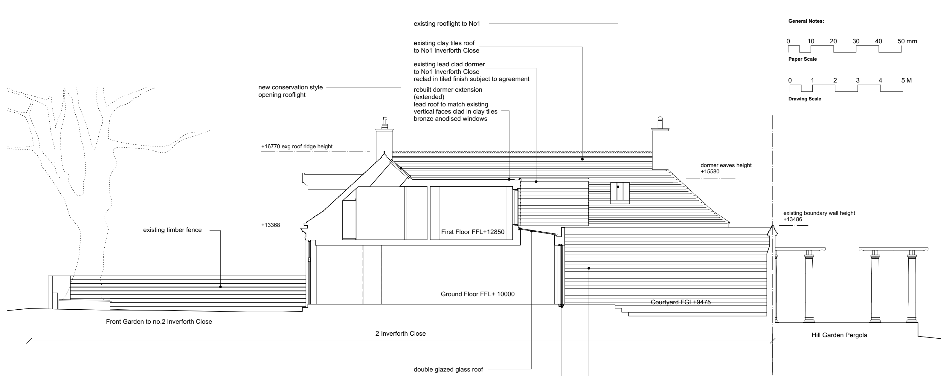
1 Proposed Courtyard West Elevation Scale: 1:100
