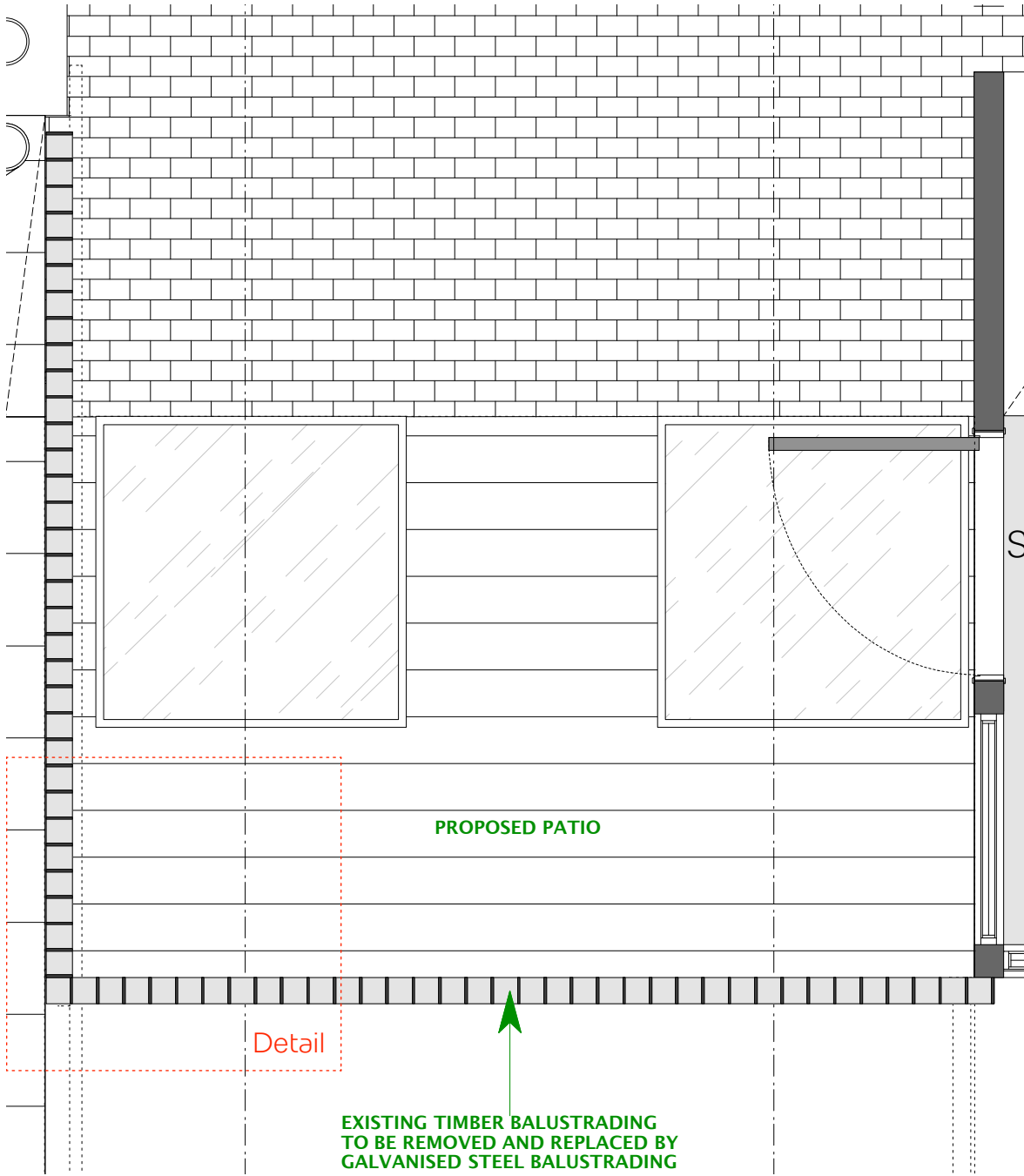
Approved Roof plan 1.25
