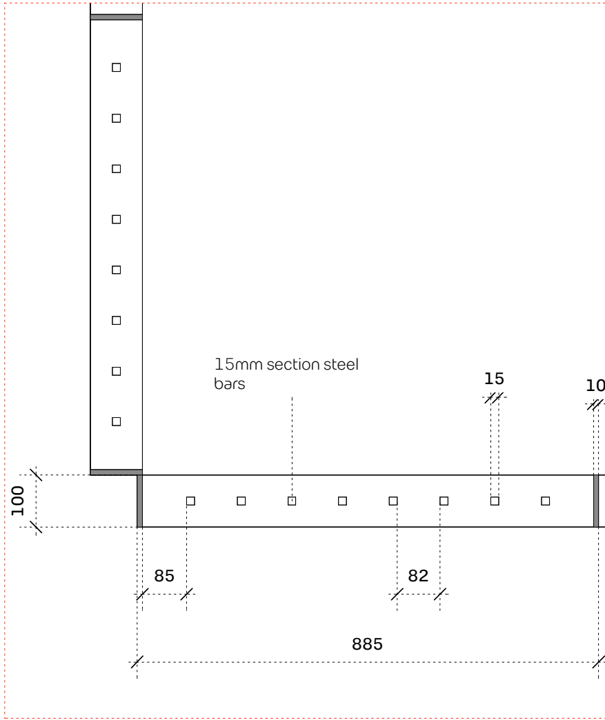
Proposed Amendment Detail 1.10 in a plan view
