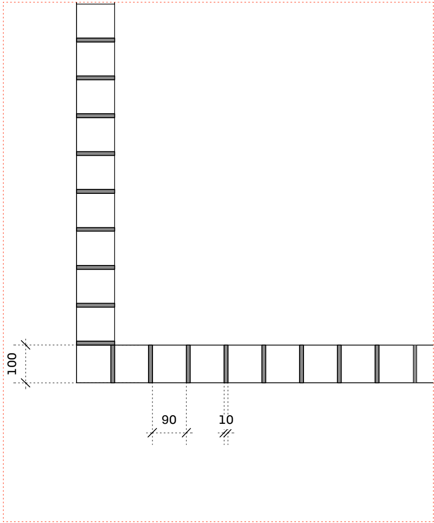
Approved Detail 1.10 in a plan view
