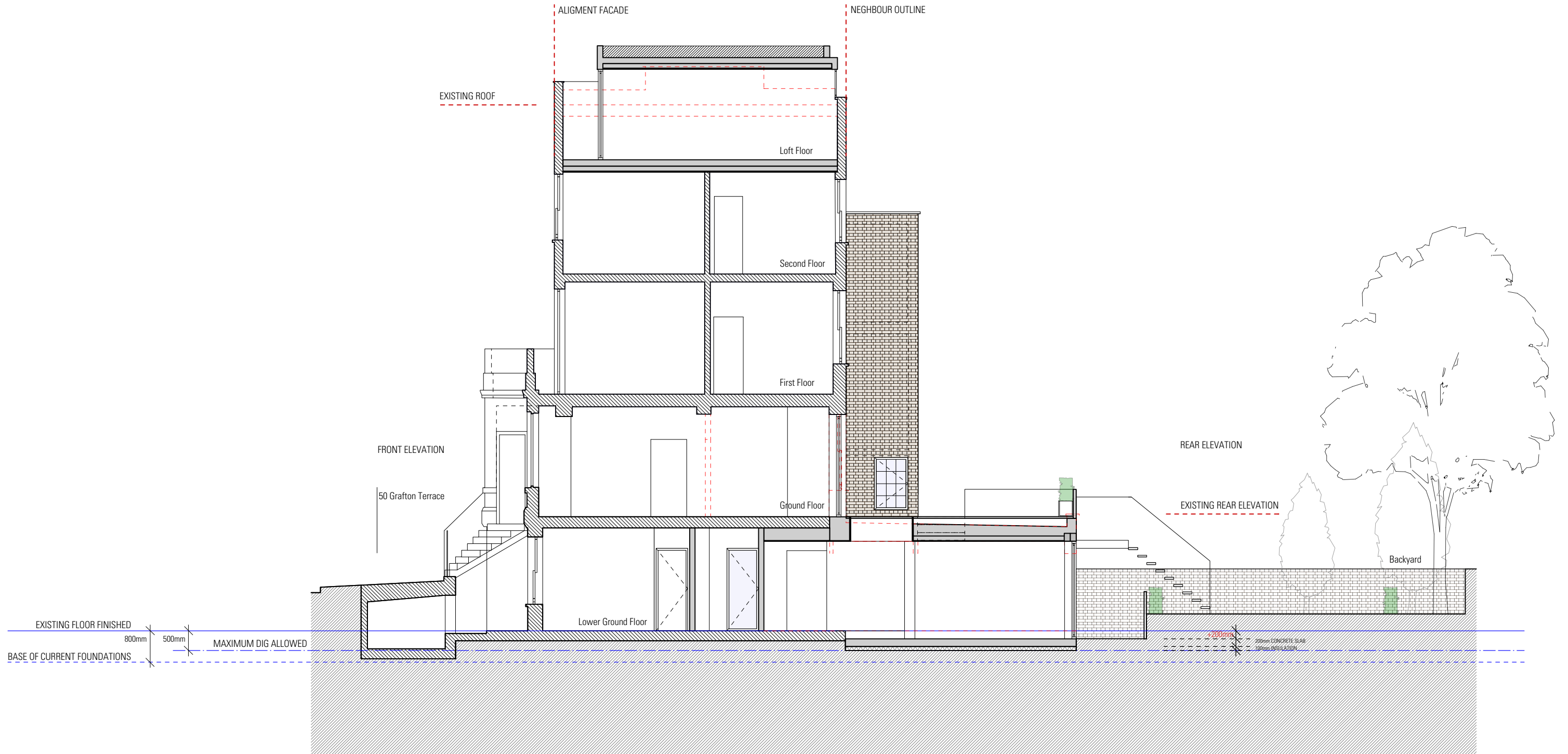
2 Long Section Scale 1:100@A3
