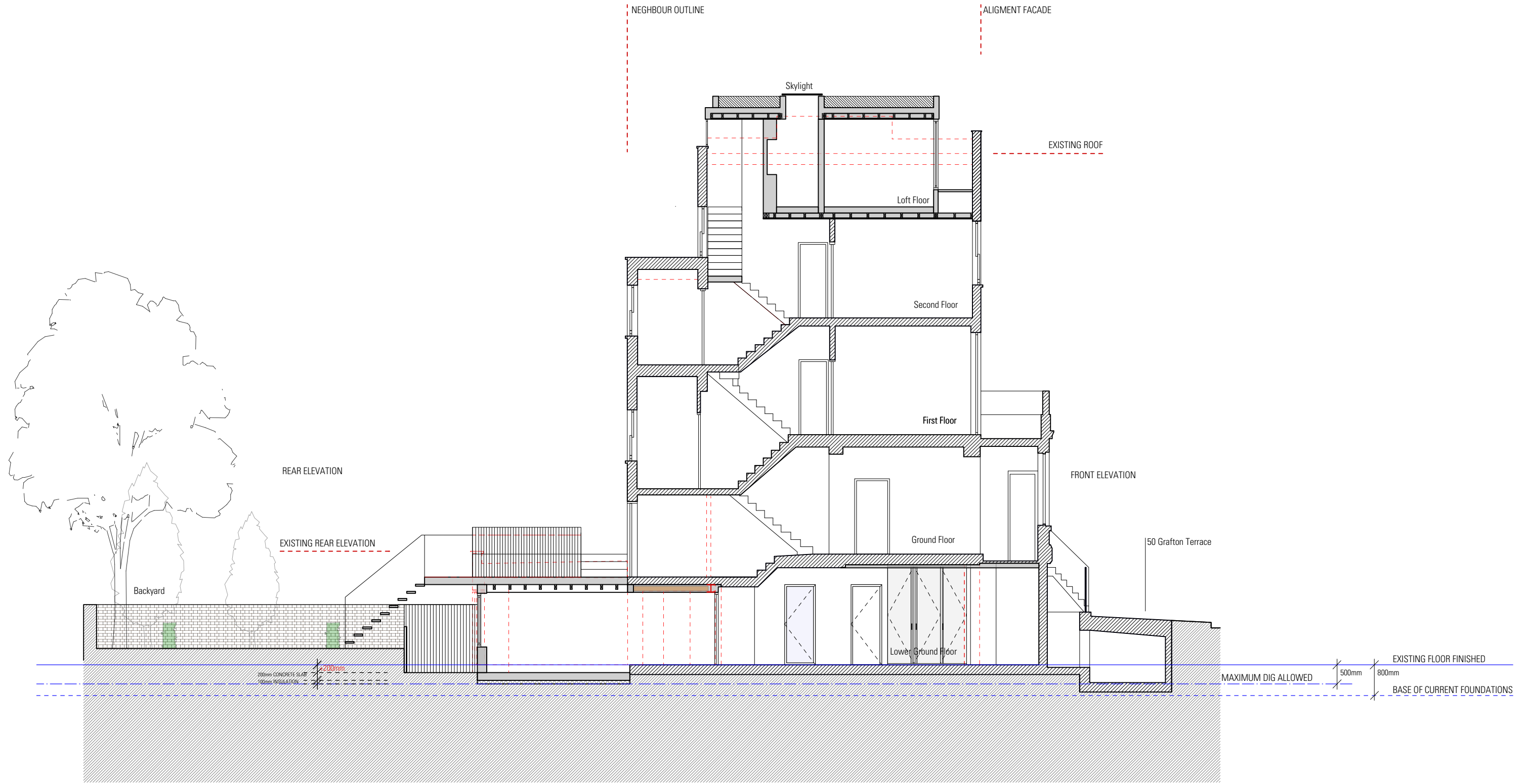
1 Long Section Scale 1:100@A3
