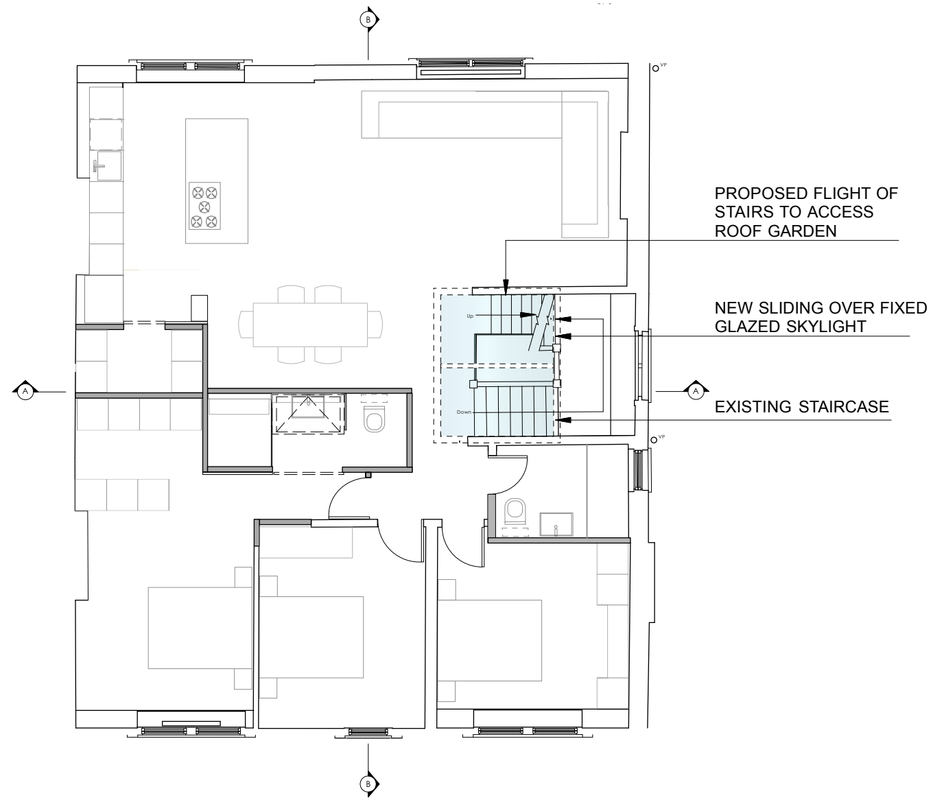
PROPOSED FLAT LAYOUT
