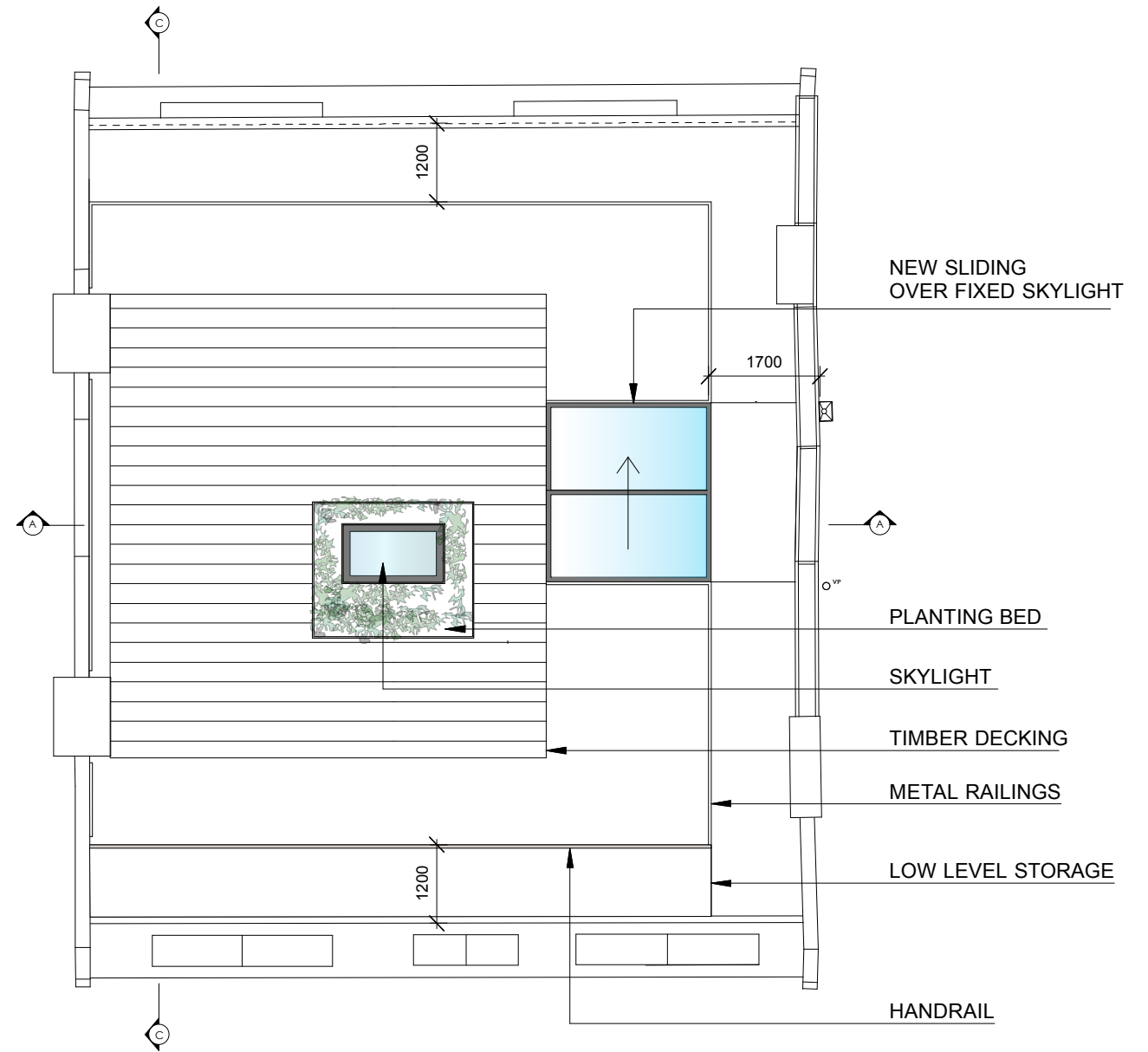
PROPOSED ROOF
