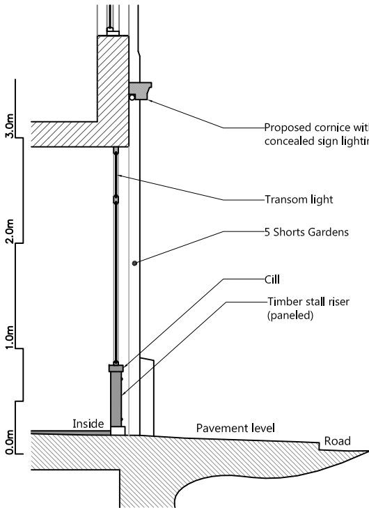
SECTION C-C AS PROPOSED @ 1:50 SCALE
