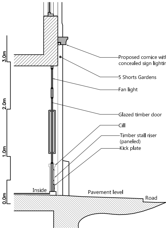
SECTION D-D AS PROPOSED @ 1:50 SCALE
