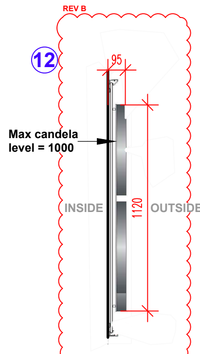
Section B-B Scale 1:20 @ A3
