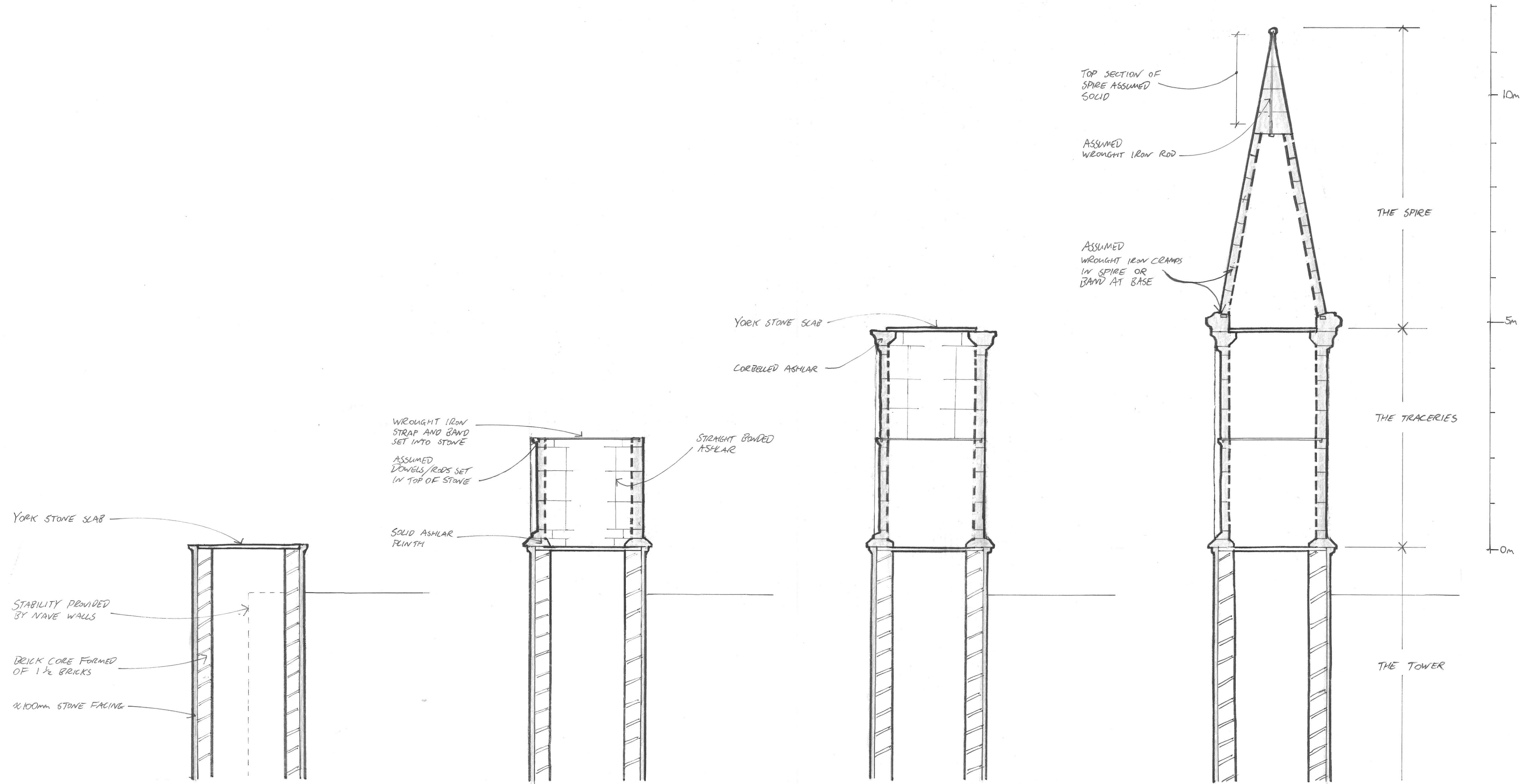
ASSUMED CONSTRUCTION SEQUENCE OF EXISTING TOWER
