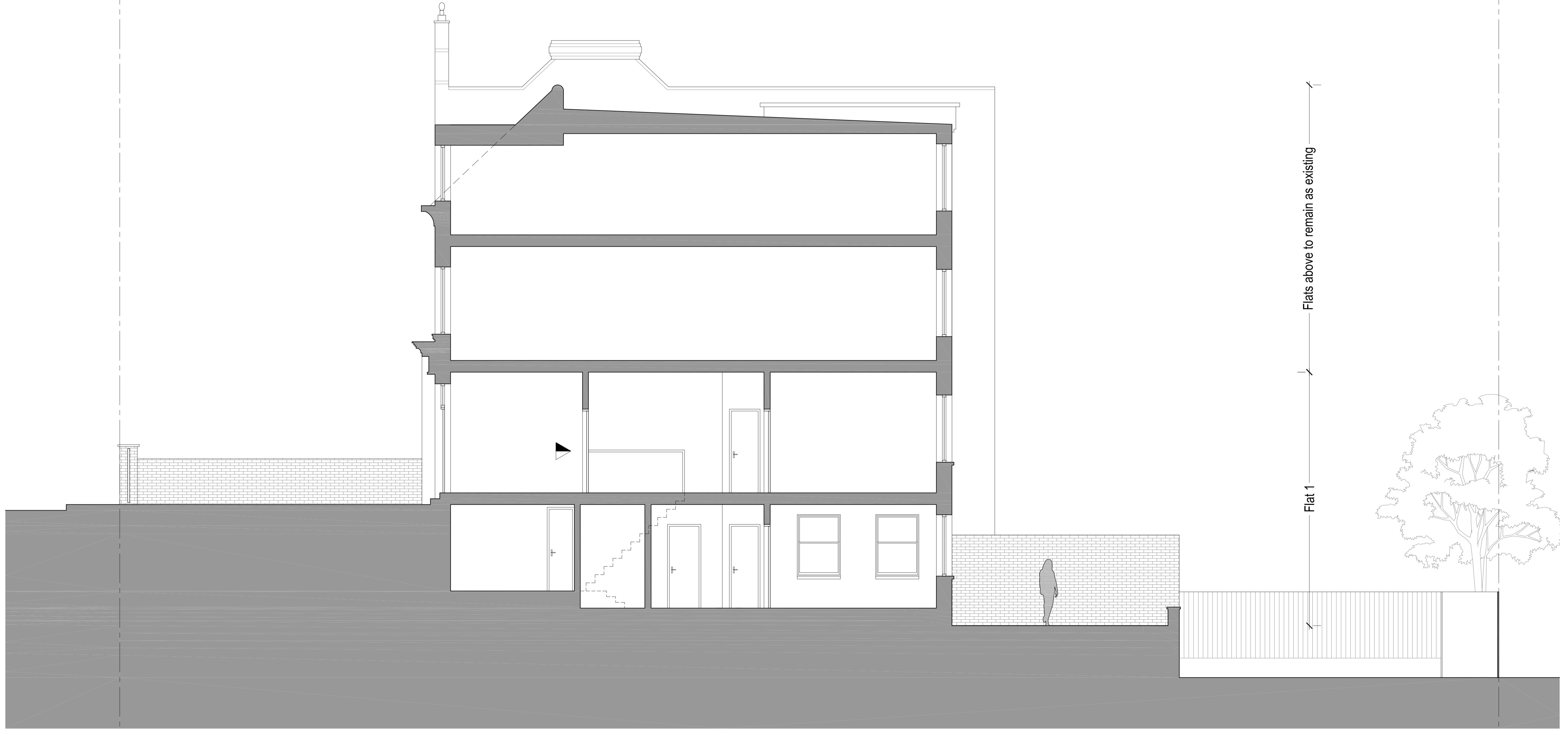
Existing Section CC Scale 1:50
