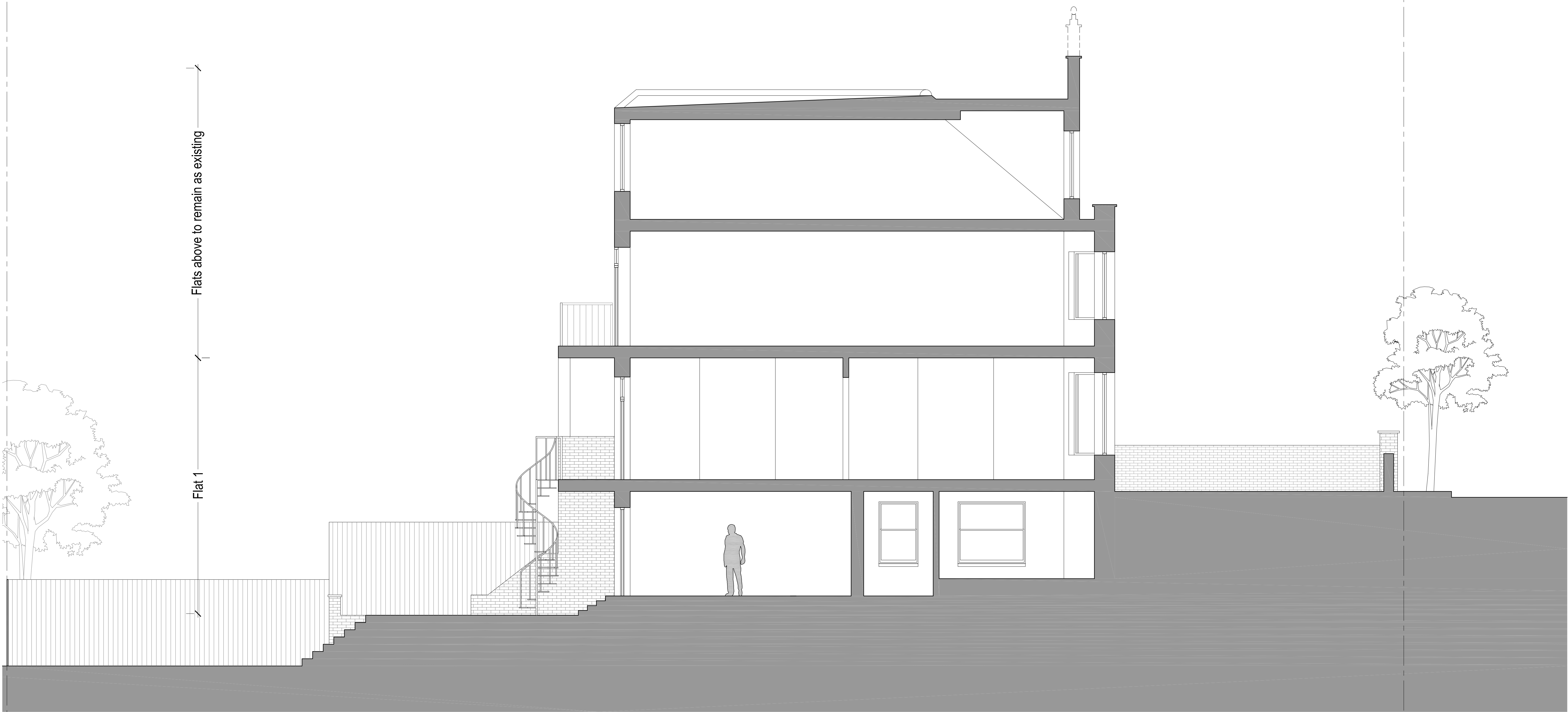
Existing Section AA Scale 1:50
