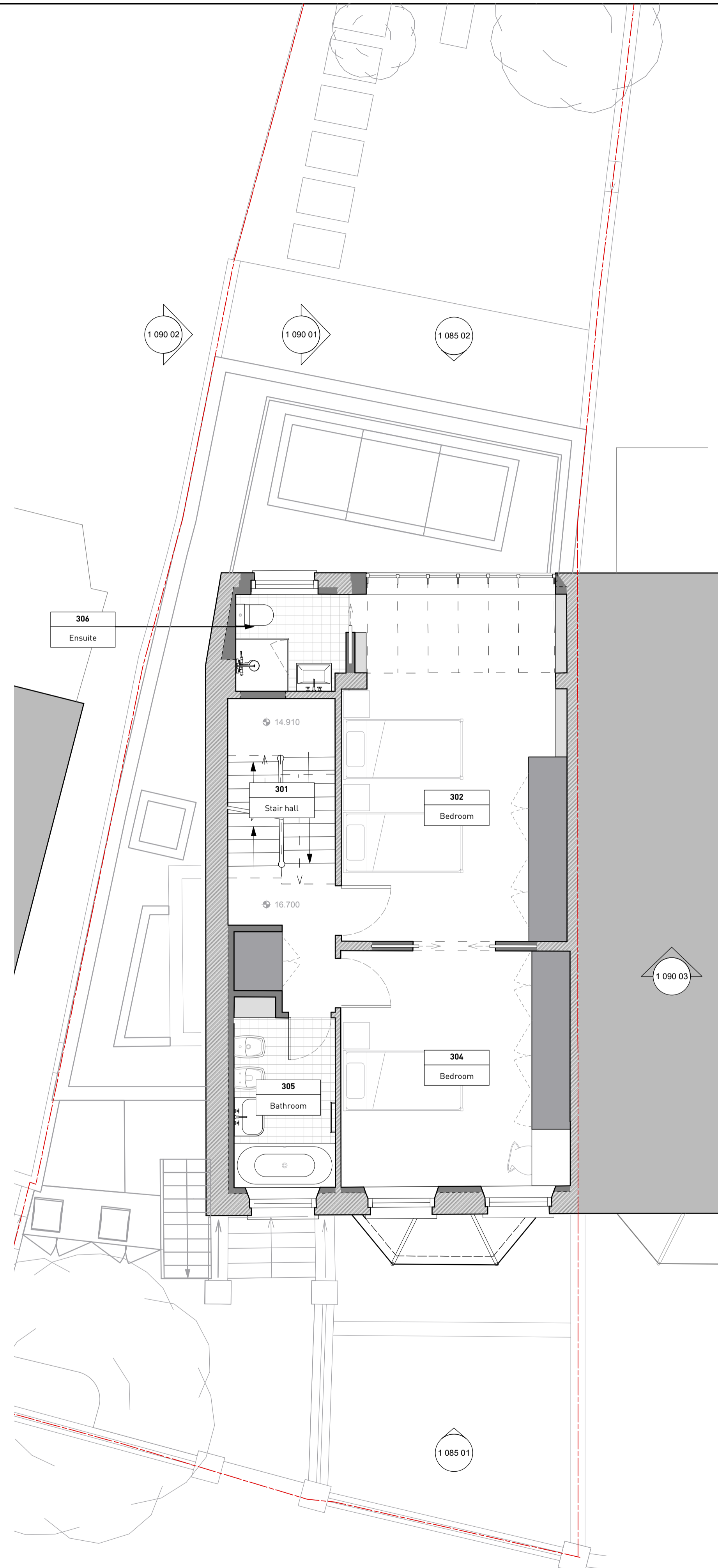
2 First floor plan - OPTION B Scale: 1:50
