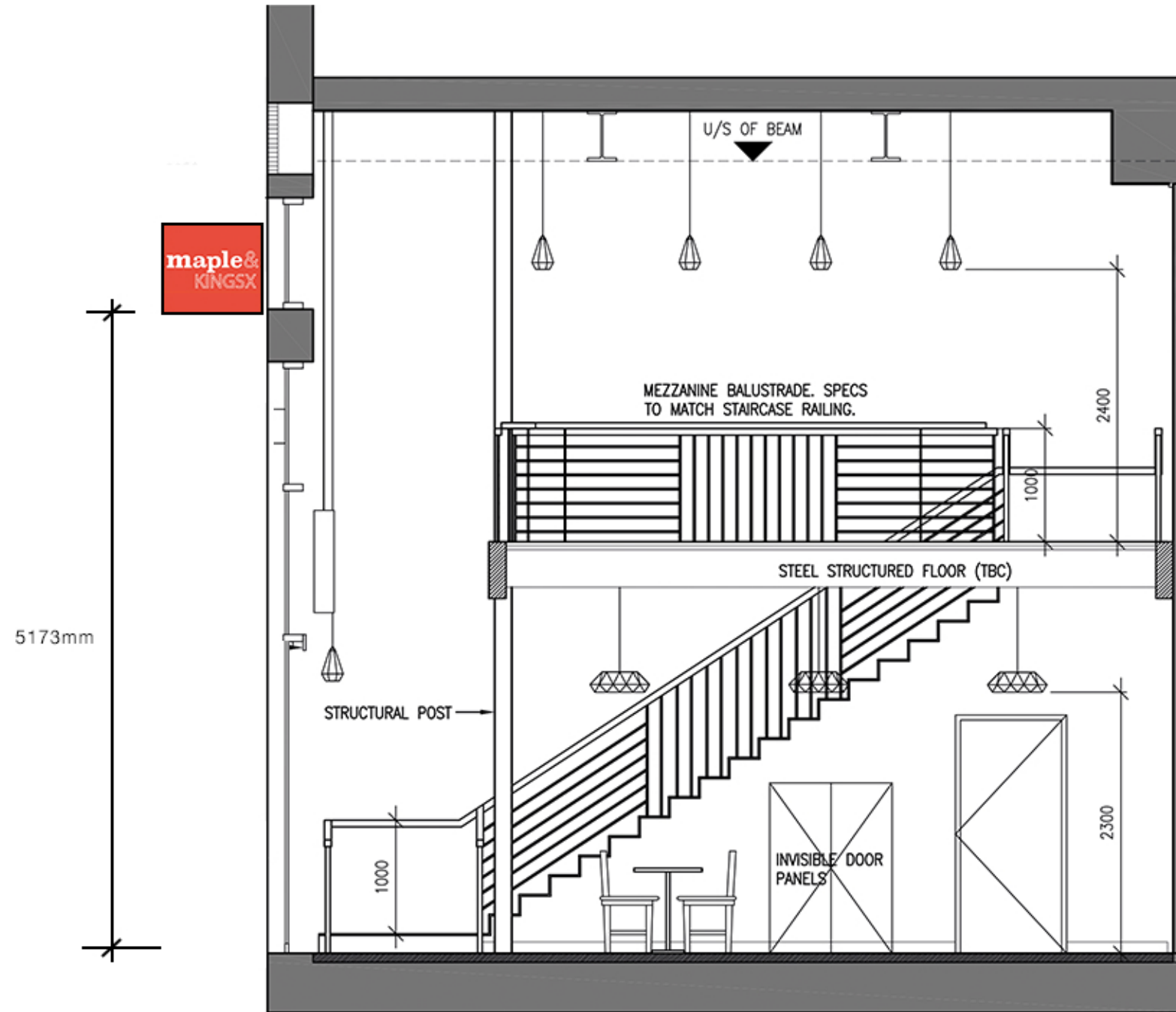
1 SECTION 1 501 SCALE 1:50 @ A3 PROPOSED
