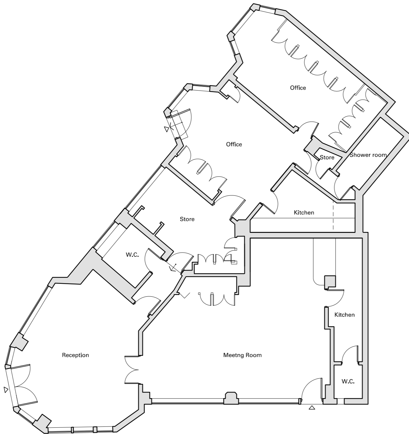
Upper Ground Floor Plan
