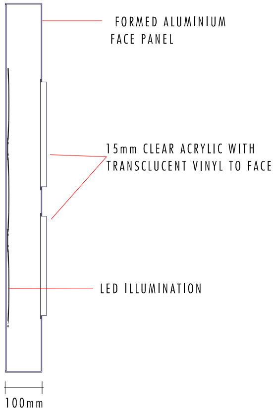
SECTION THROUGH SIGN A Scale 1:10
