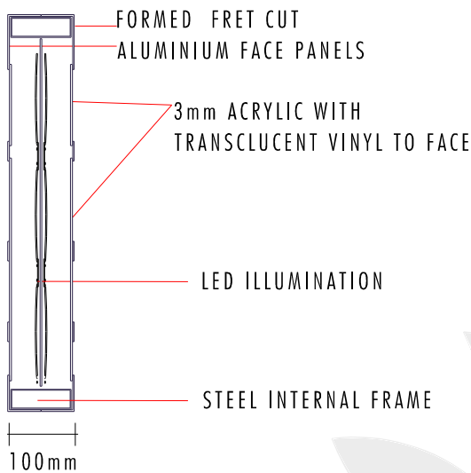
SECTION THROUGH SIGN B Scale 1:10
