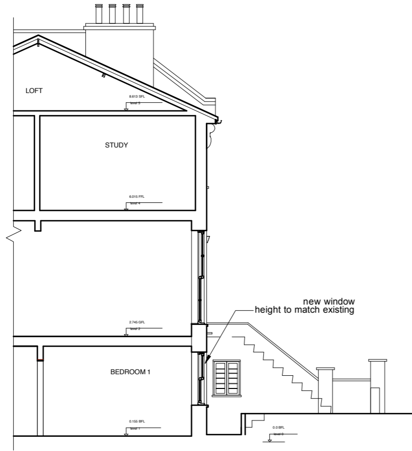
PROPOSED SECTION A
