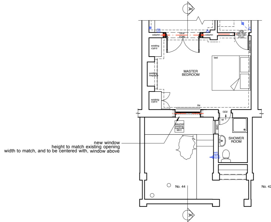
PROPOSED LOWER GROUND FLOOR PLAN
