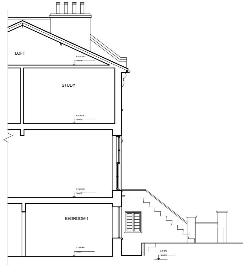
EXISTING SECTION
