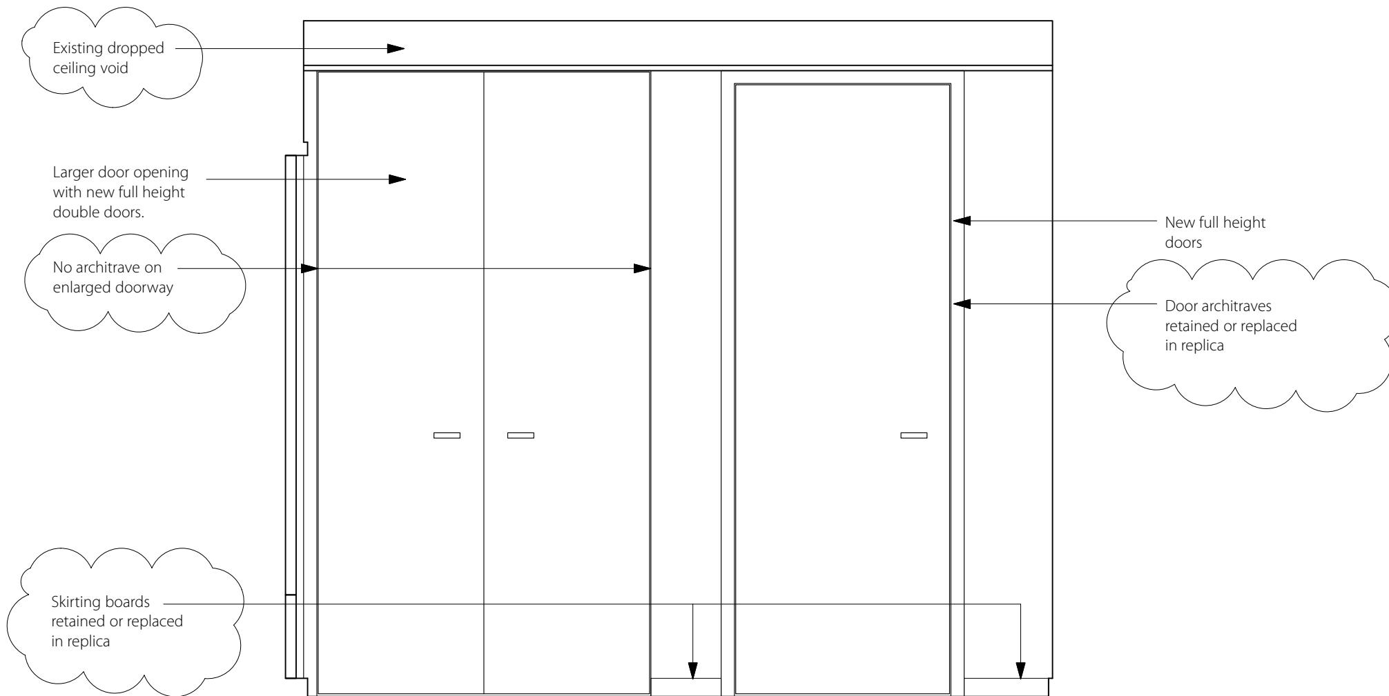
ELEVATION C
