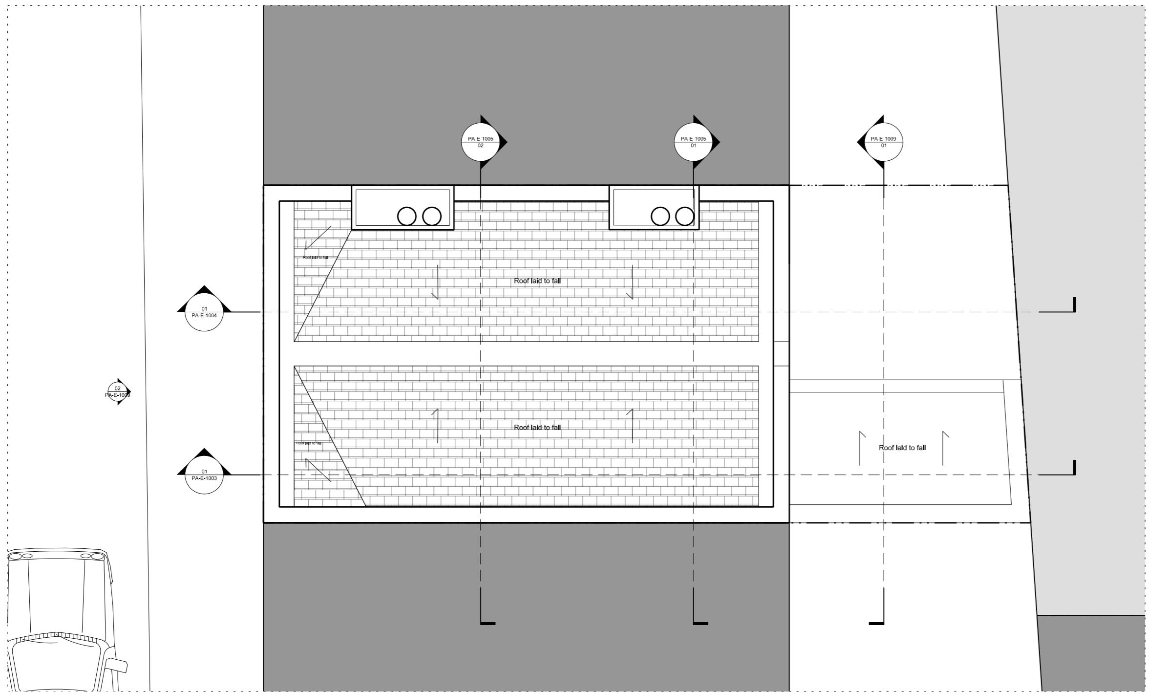
01 ROOF PLAN 1:50
